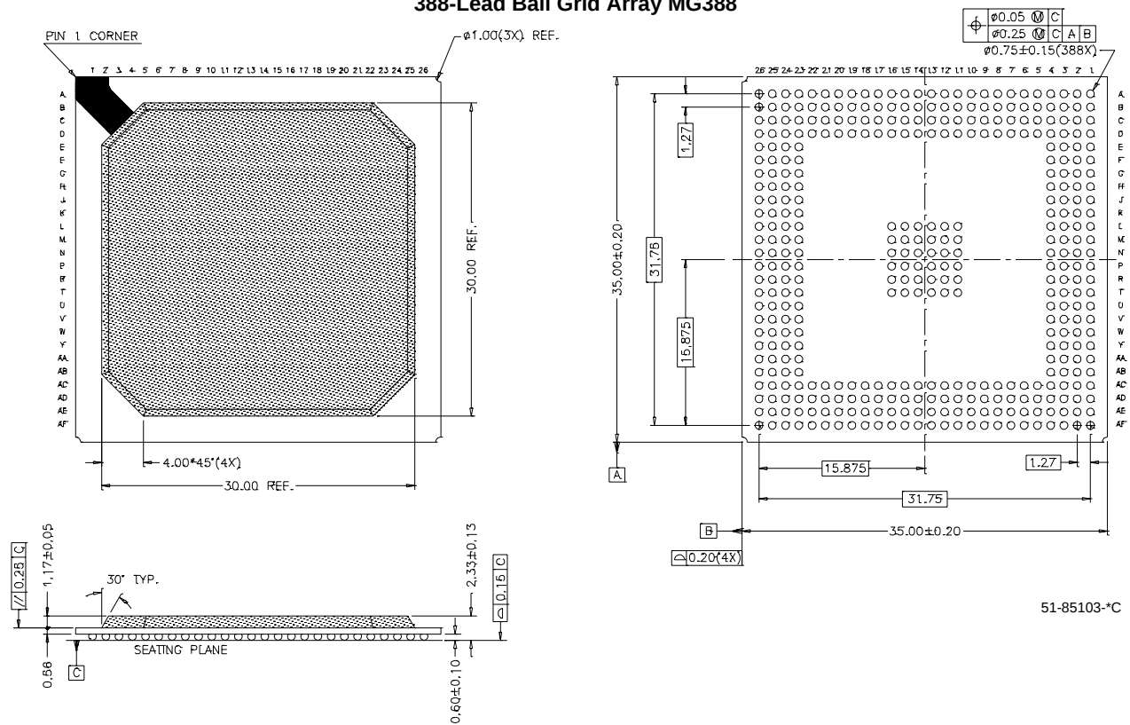
388-Lead Ball Grid Array MG388
