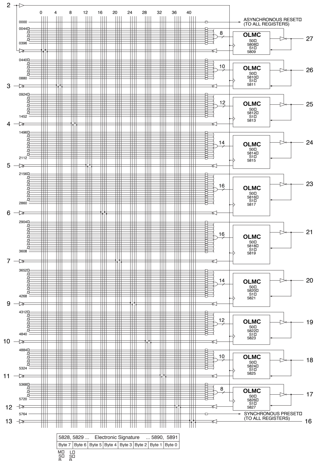
PLCC Package Pinout
