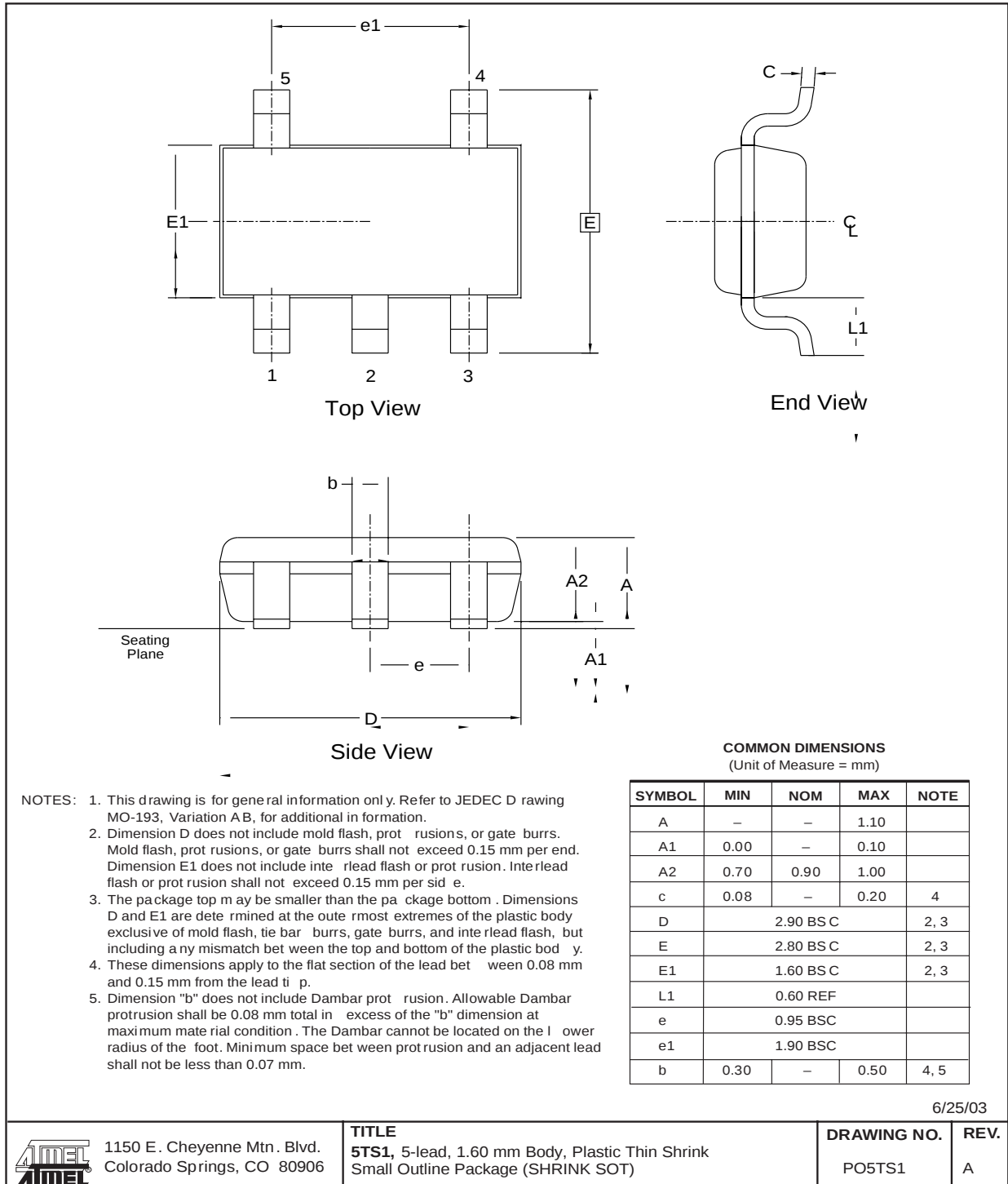
Figure 19. 5TS1 – SOT23
