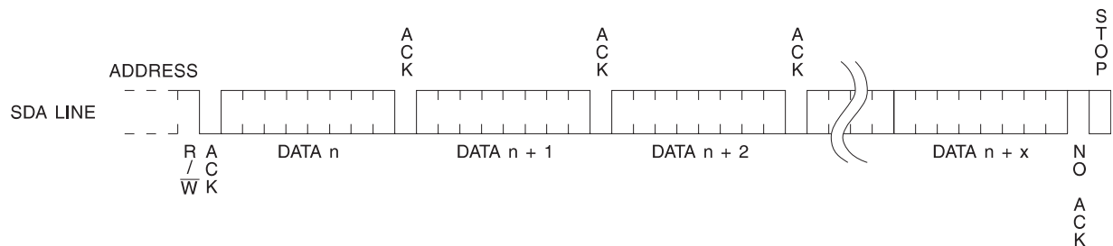
Figure 10. Sequential Read
