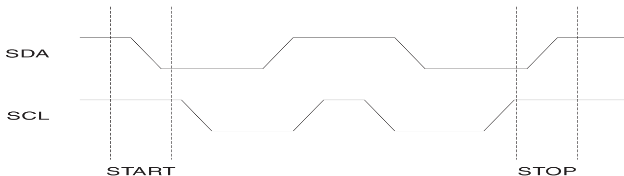
Figure 5. Start and Stop Definition
