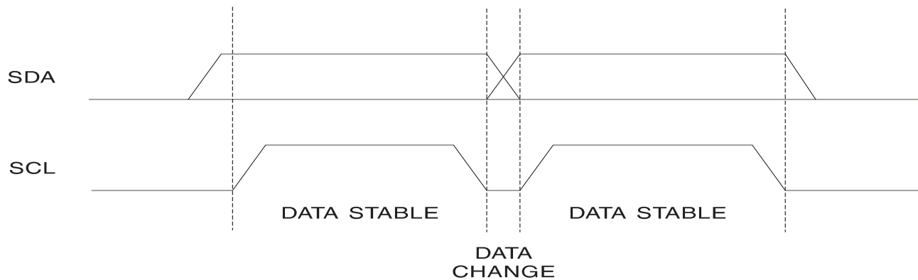
Figure 4. Data Validity
