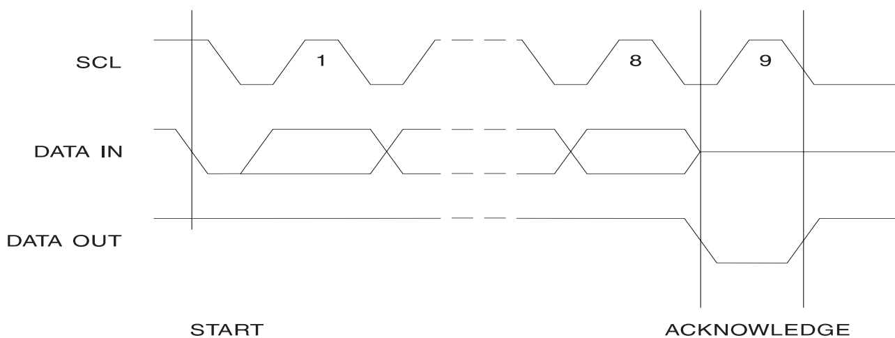
Figure 6. Output Acknowledge
