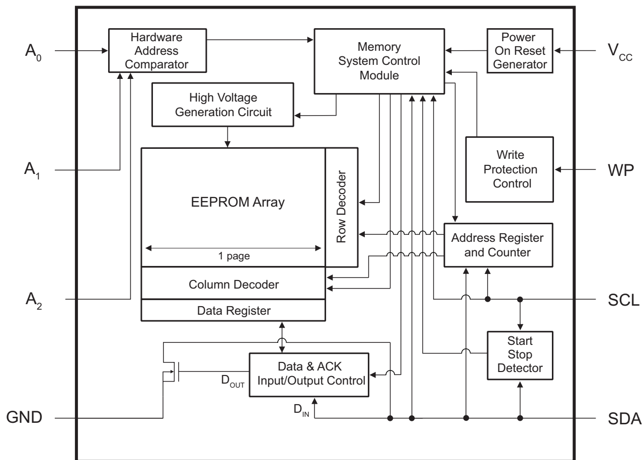
Figure 2-1. Block Diagram
