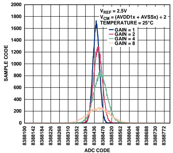
Figure 19. Noise Histogram at 2 kSPS, Low Power Mode
