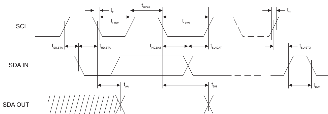
Figure 6-5. Bus Timing
