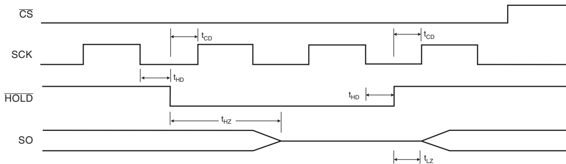
Figure 10. HOLD Timing
