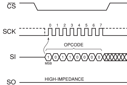
Figure 8-9. Program/Erase Suspend
