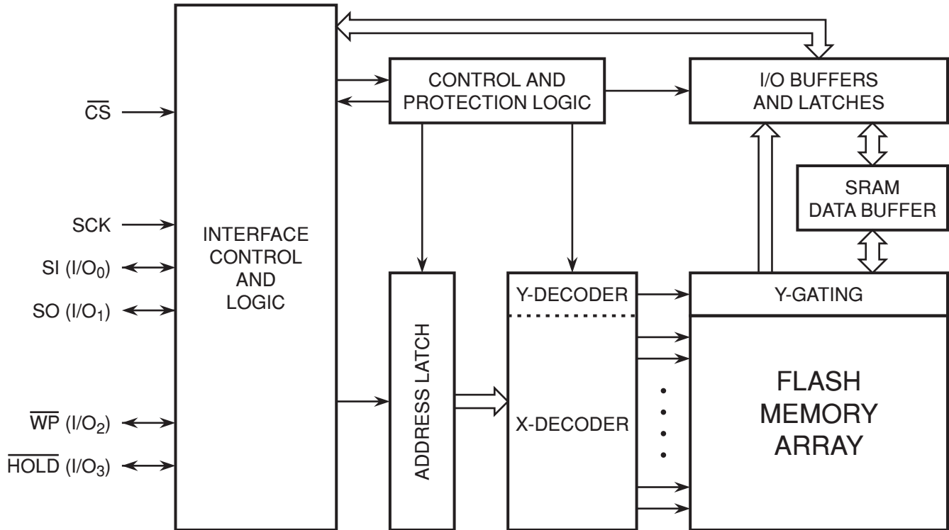
Figure 3-1. Block Diagram
