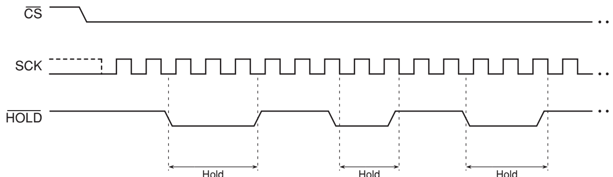
Figure 12-5. Hold Mode
