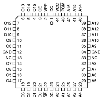
PLCC Top View
