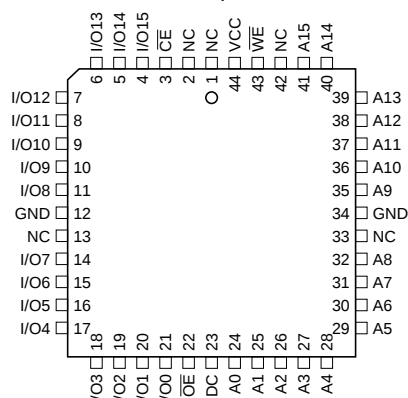
PLCC Top View
