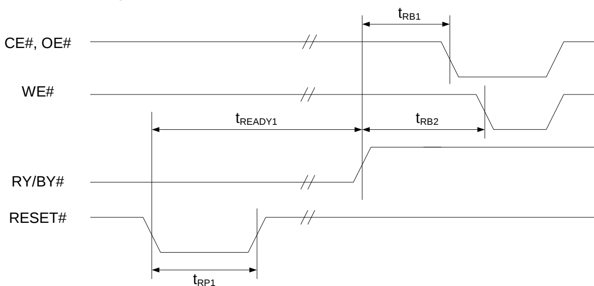
Figure 1. AC Waveforms for RESET# Reset# Timings
