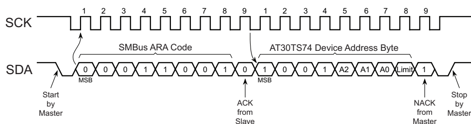
Figure 6-1. SMBus Alert
