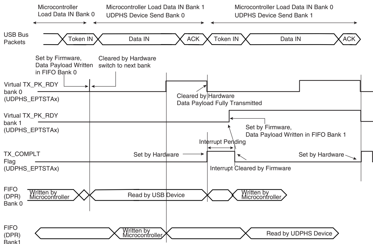
Figure 31-8. Data IN Transfer for Endpoint with Two Banks
