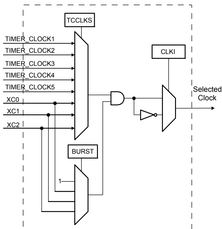
Figure 32-2. Clock Selection
