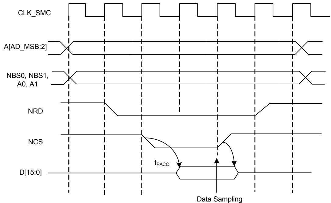
Figure 18-10. READMODE = 0: Data Is Sampled by SMC Before the Rising Edge of NCS
