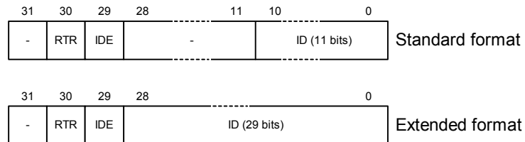
Figure 29-8. Identifier Tag (IDT)
