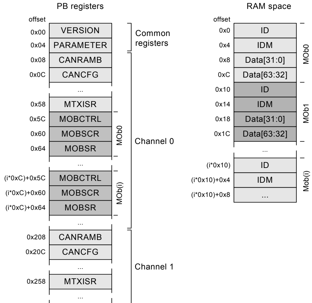
Figure 29-12. Address Map Overview
