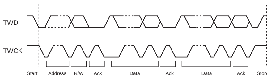
Figure 27-4. Transfer Format
