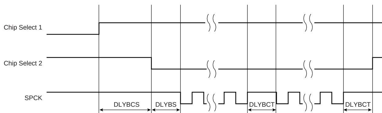
Figure 26-7. Programmable Delays
