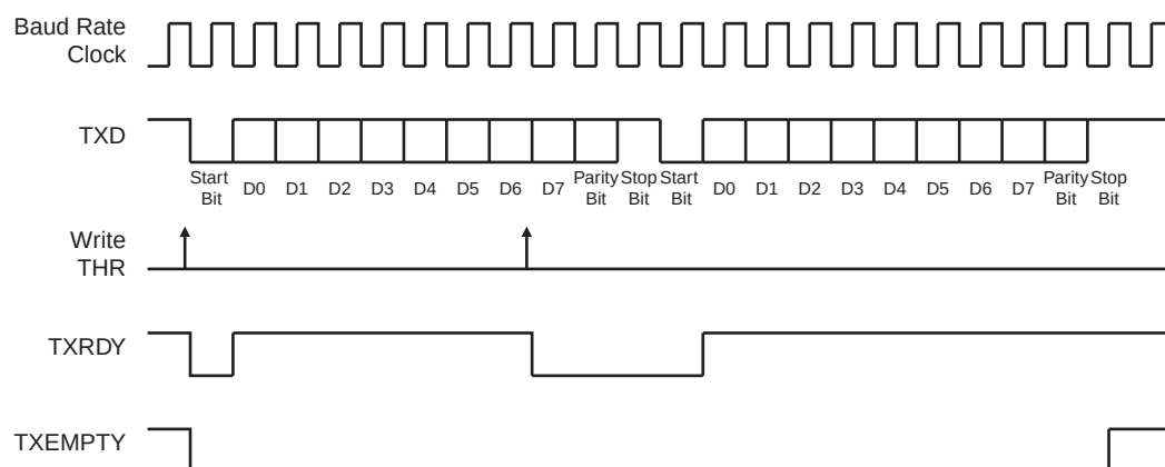
Figure 25-6. Transmitter Status
