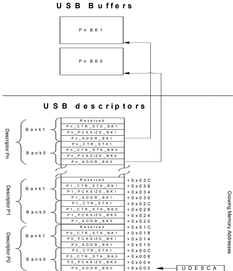
Figure 32-18. Memory organization
