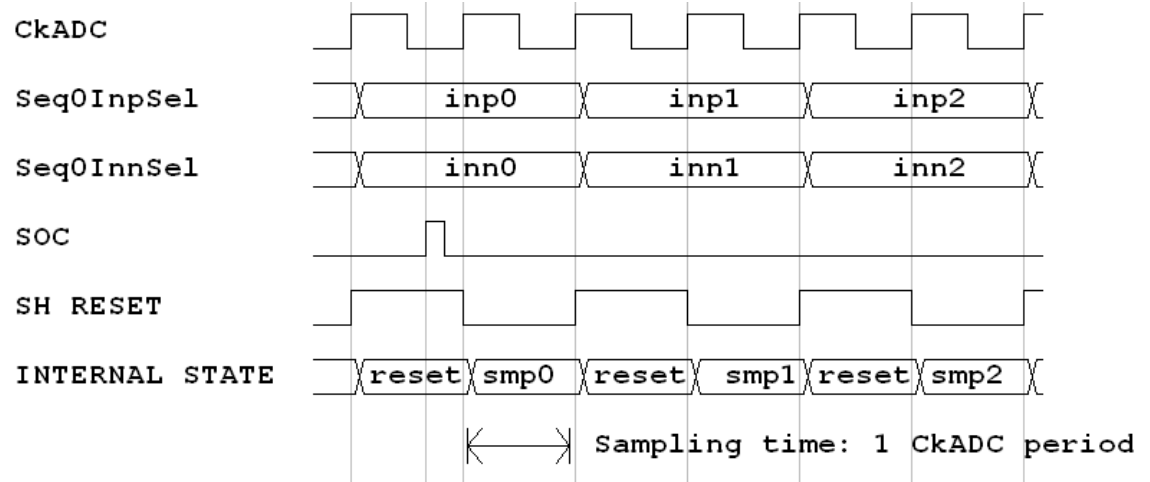
Figure 36-9. SH Dynamic Mode
