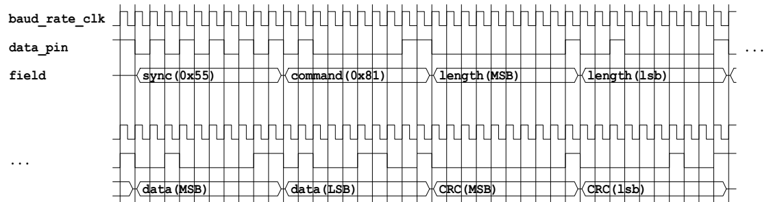
Figure 39-9. Example Command
