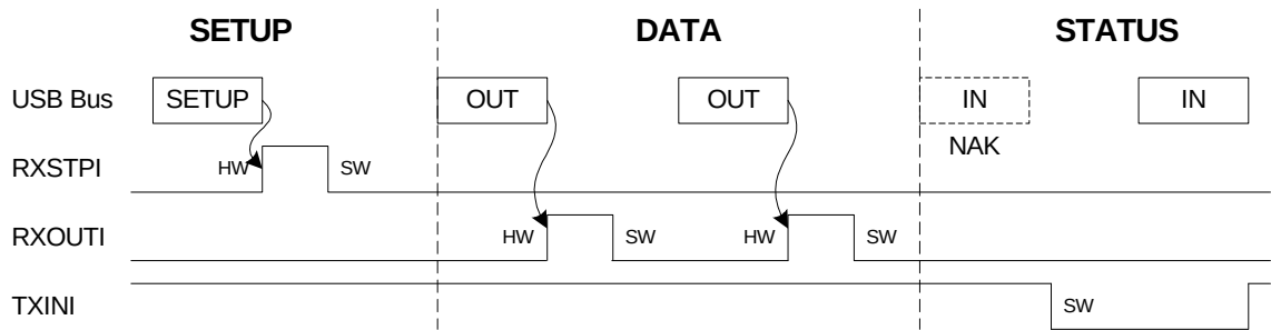
Figure 32-9. Control Write
