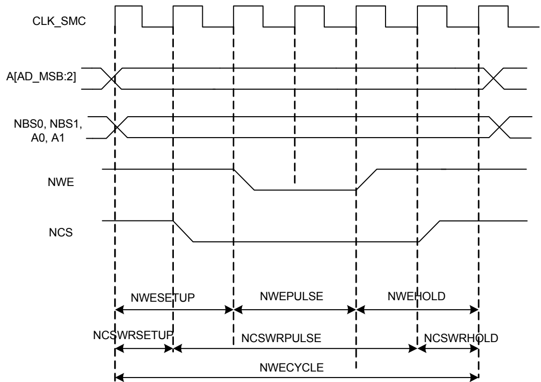
Figure 18-11. Write Cycle
