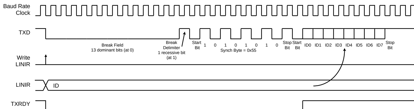
Figure 25-39. Header Transmission
