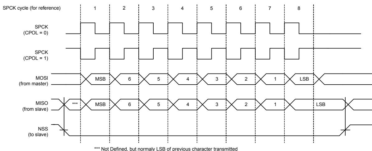
Figure 26-4. SPI Transfer Format (NCPHA = 0, 8 bits per transfer)
