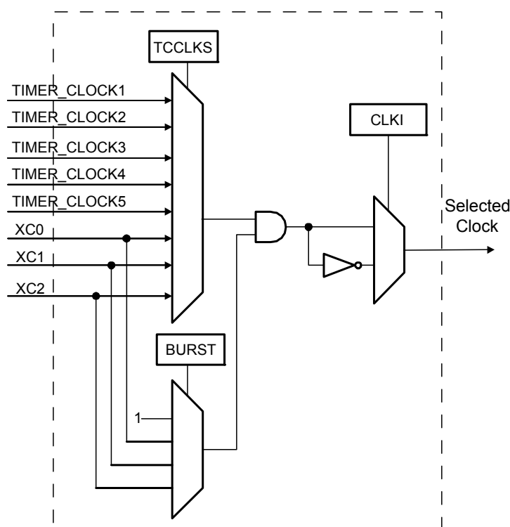
Figure 31-2. Clock Selection
