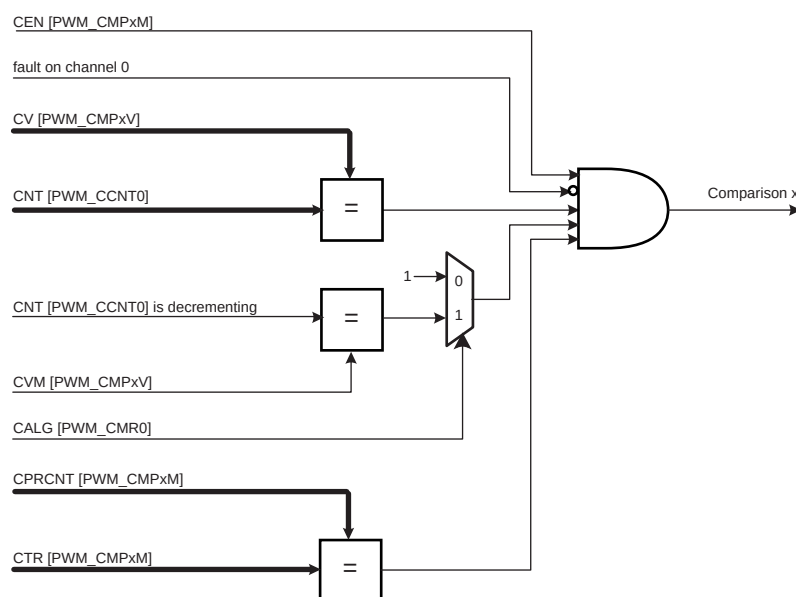
Figure 33-14. Comparison Unit Block Diagram
