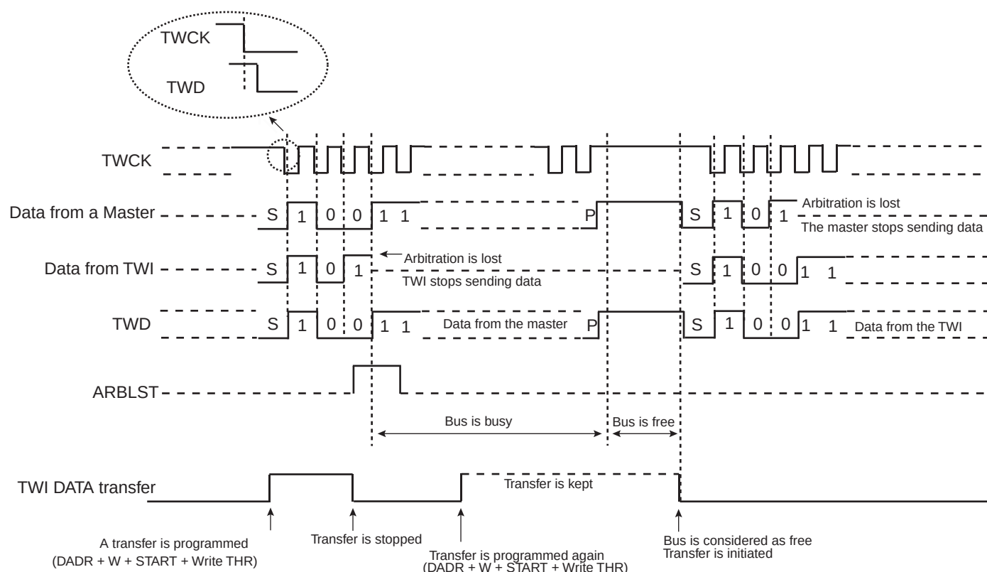
Figure 27-11. Arbitration Cases
