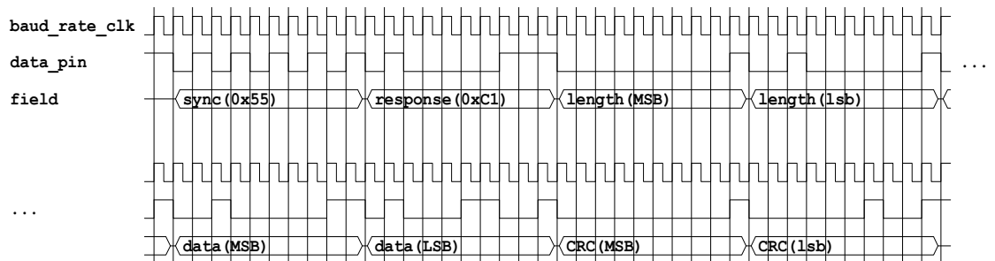
Figure 39-10. Example Response
