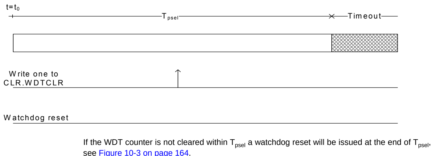
Figure 10-3. Basic Mode WDT Timing Diagram, no clear within T_{psel} .
