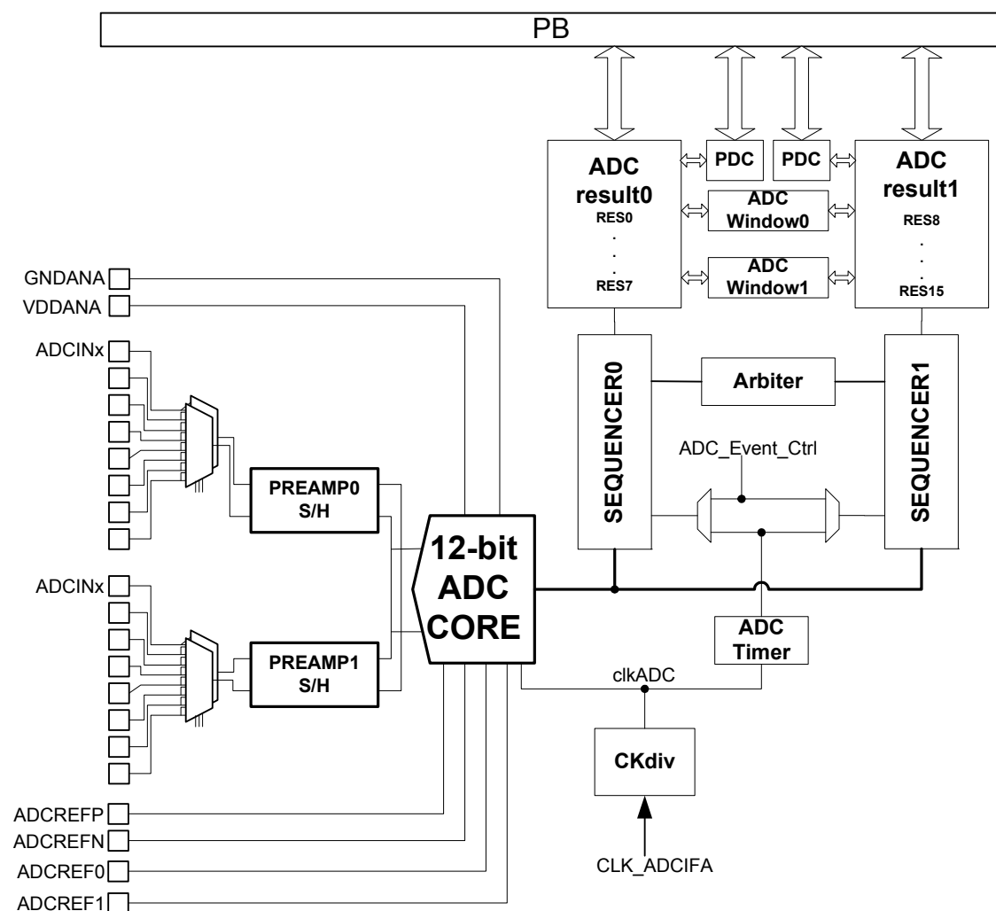
Figure 36-1. ADCIFA Block Diagram
