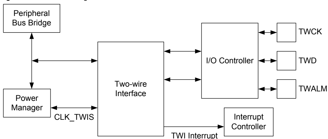
Figure 28-1. Block Diagram
