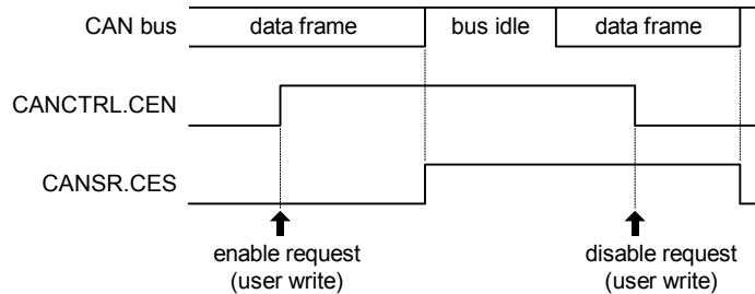
Figure 29-5. Enable and Disable Sequences
