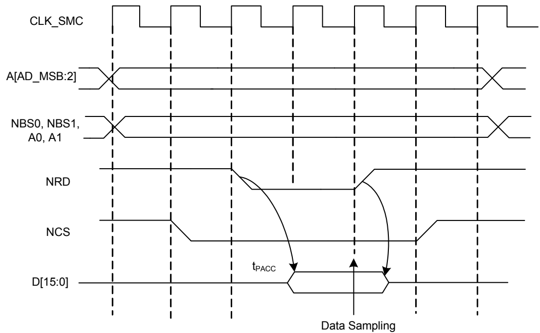
Figure 18-9. READMODE = 1: Data Is Sampled by SMC Before the Rising Edge of NRD
