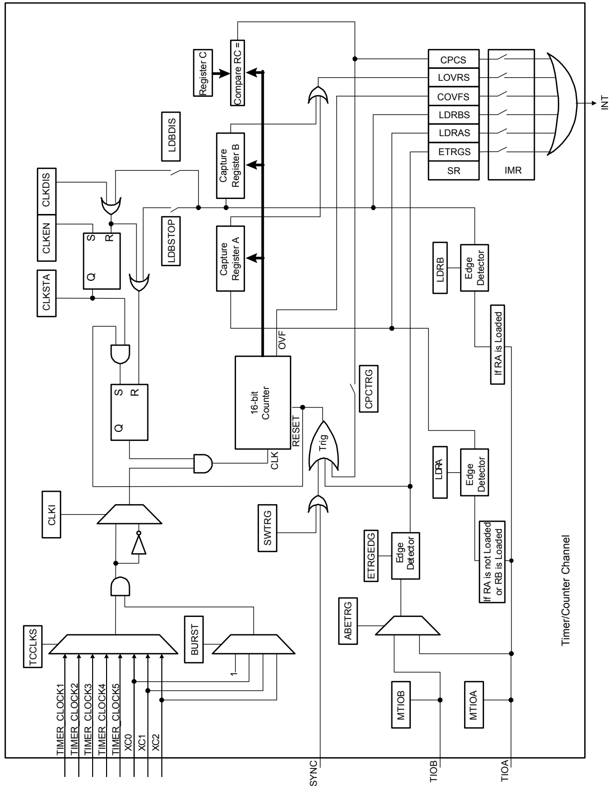
Figure 31-4. Capture Mode
