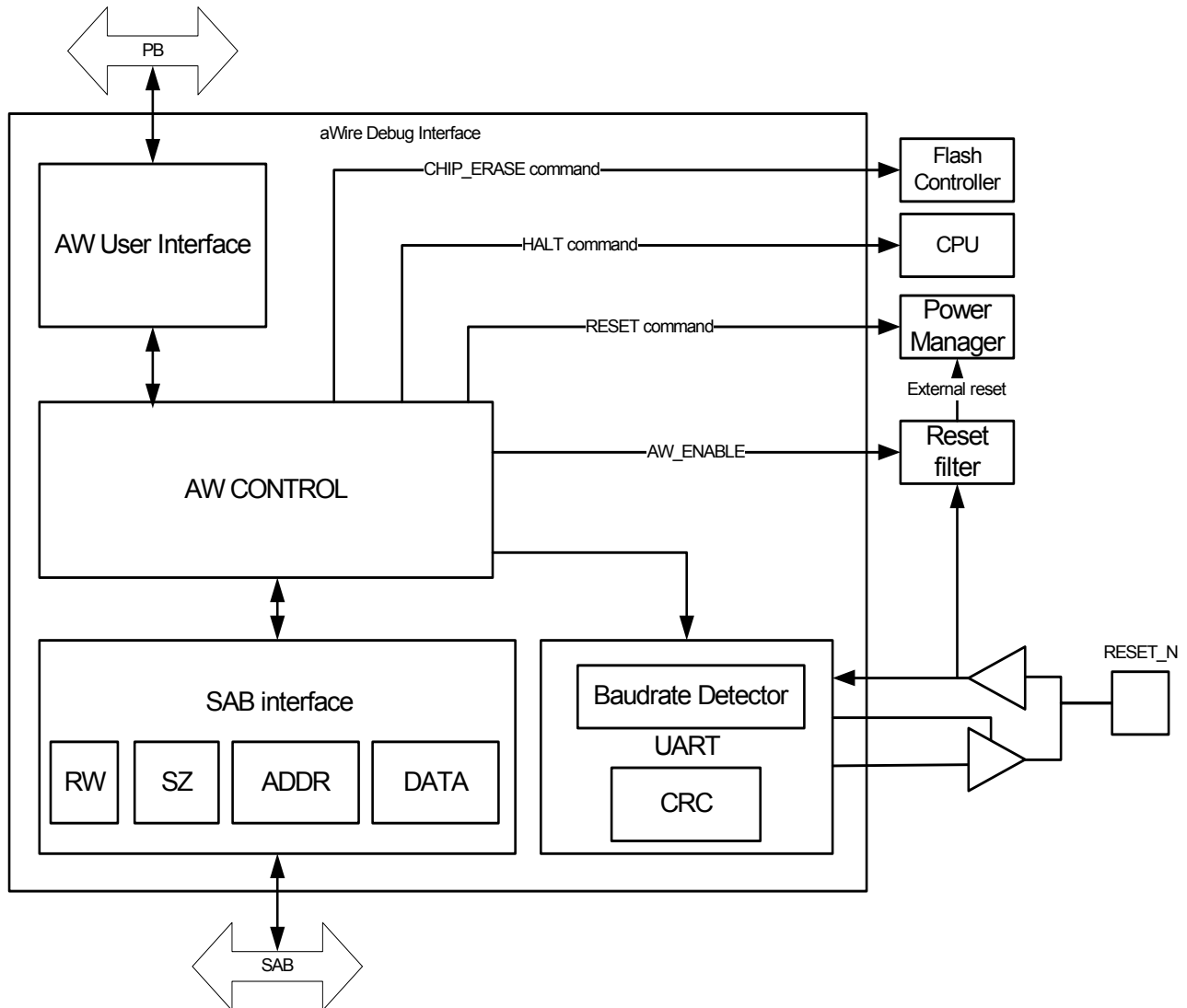
Figure 39-8. aWire Debug Interface Block Diagram
