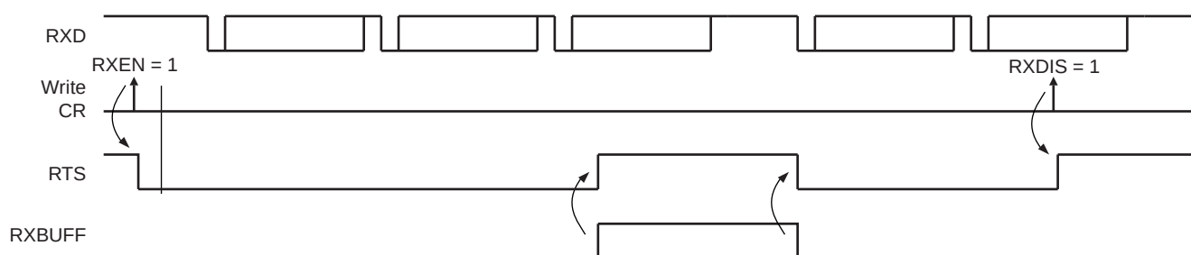
Figure 25-27. Receiver Behavior when Operating with Hardware Handshaking
