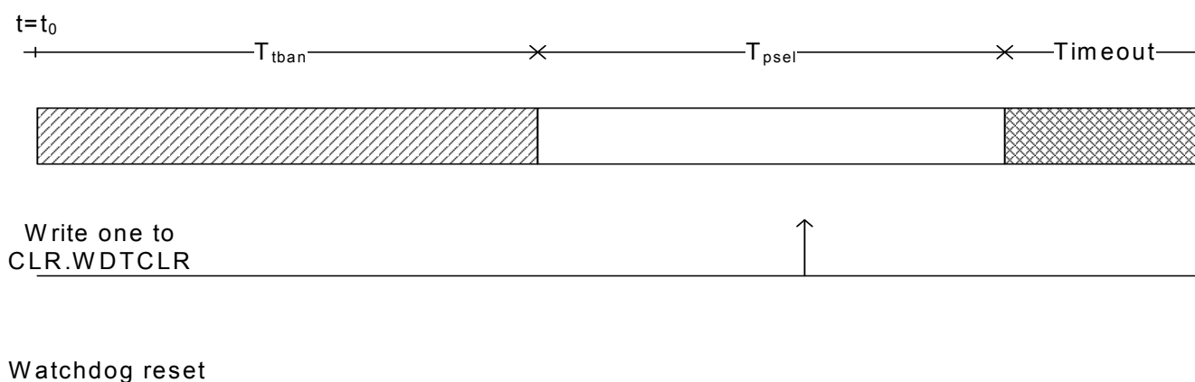
Figure 10-4. Window Mode WDT Timing Diagram
