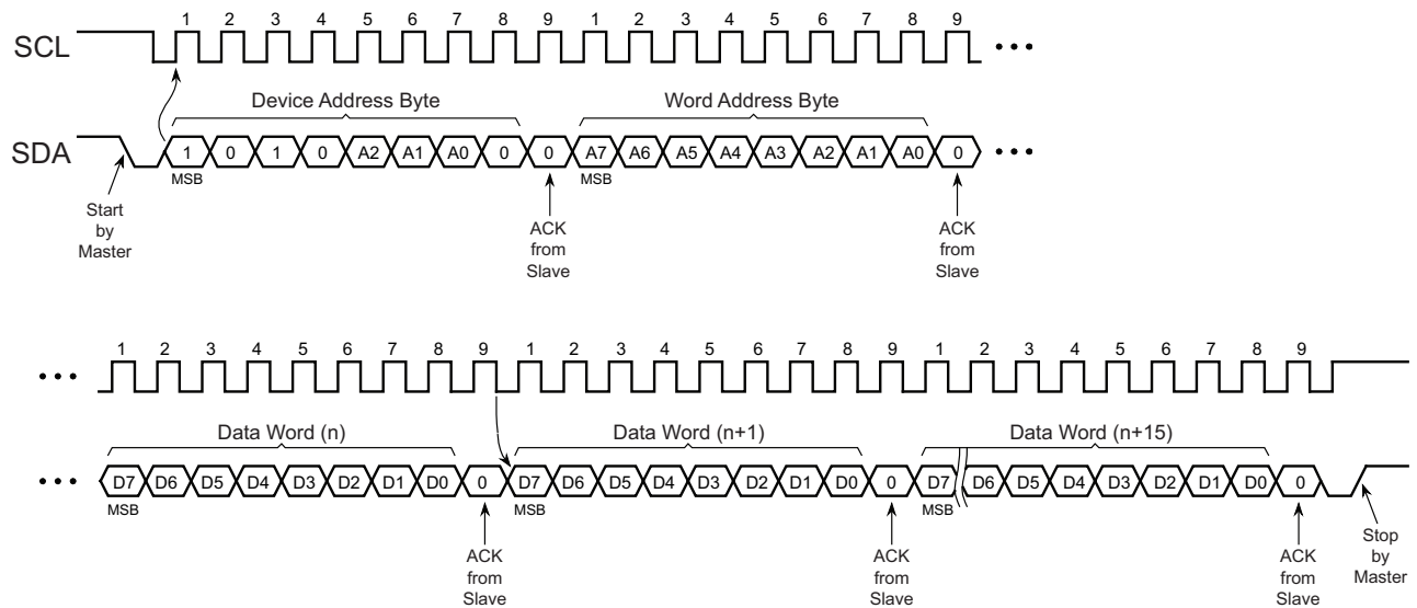
Figure 6-7. Page Write
