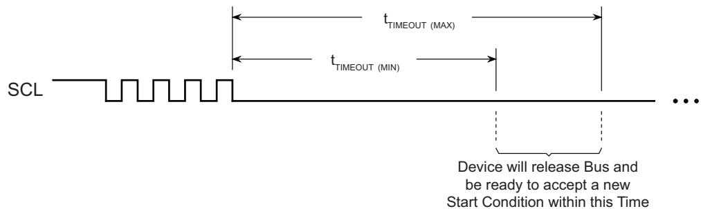
Figure 3-3. Timeout
