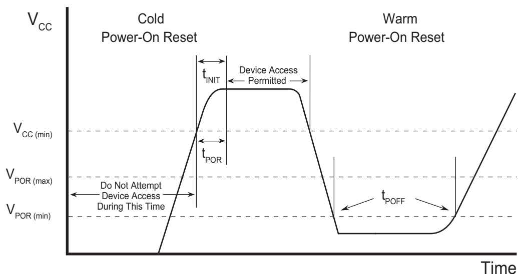
Figure 3-2. Power-up Timing
