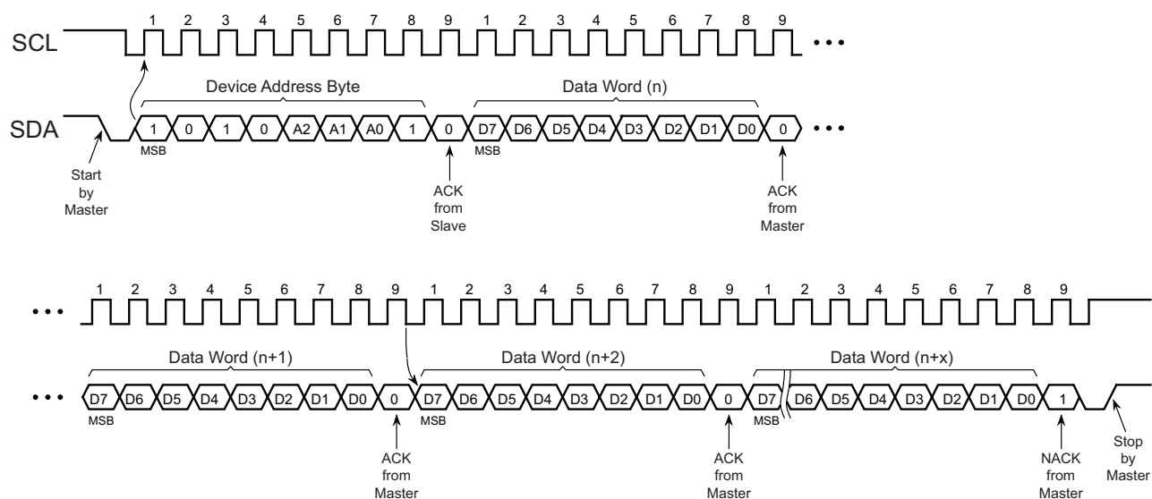
Figure 6-5. Sequential Read
