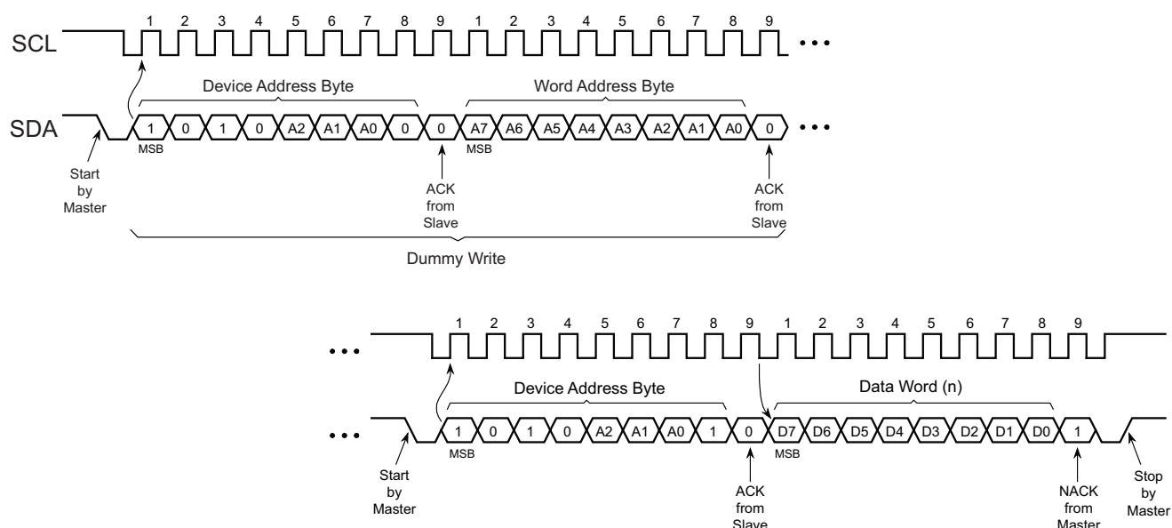
Figure 6-4. Random Read
