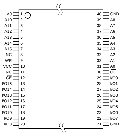
AT49BV/LV1024A VSOP Top View
