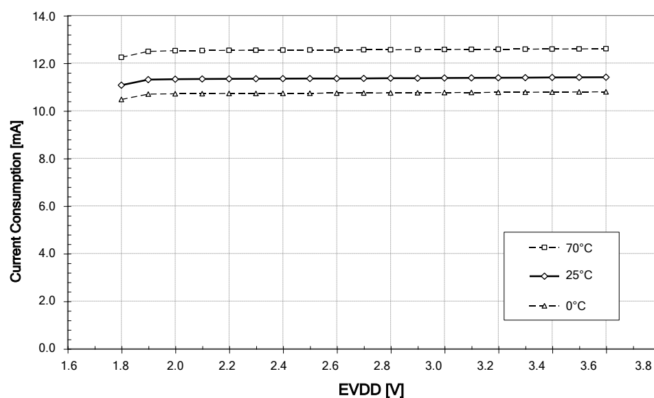
Figure 13-5. Current Consumption in RX_ON State – Reduced Sensitivity.
