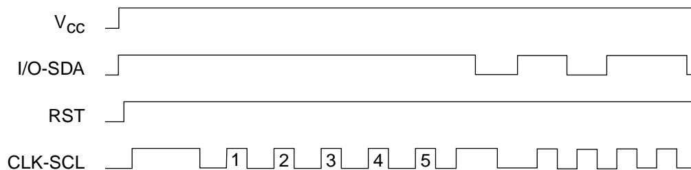
Figure 6-1. Asynchronous Mode
