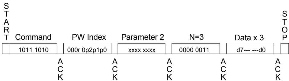
Figure 8-18. Verify Password
