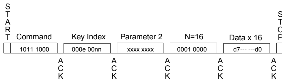
Figure 8-16. Verify Crypto
