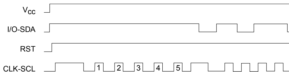
Figure 7-1. Asynchronous Mode
