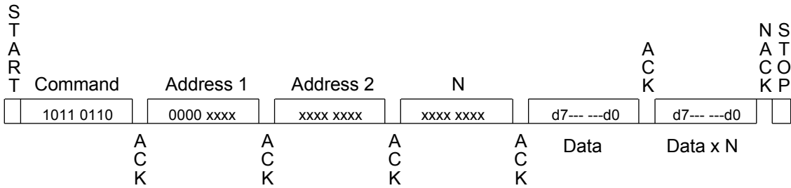
Figure 8-14. System Read
