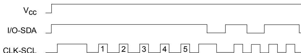
Figure 8-1. Start-up Sequence
