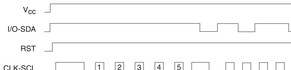
Figure 8. Synchronous 2-wire Protocol
