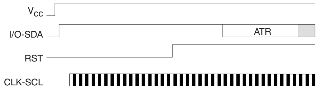
Figure 7. Asynchronous T = 0 Protocol (Gemplus Patent)
