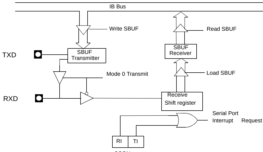
Figure 20. Serial I/O Port Block Diagram
