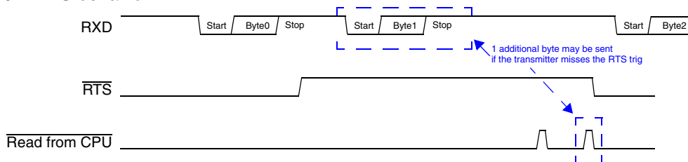
Figure 17-9. \overline{\text{RTS}} behavior
