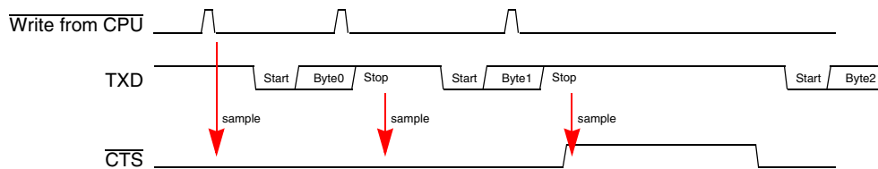
Figure 17-10. \overline{\text{CTS}} behavior
