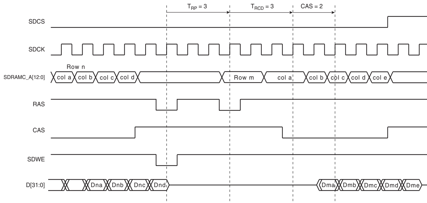
Figure 21-4. Read Burst with Boundary Row Access
