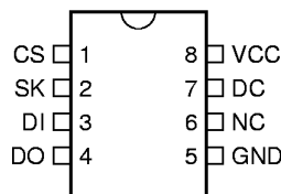
8-Pin PDIP
