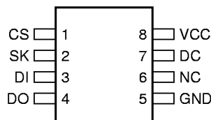
8-Pin SOIC
