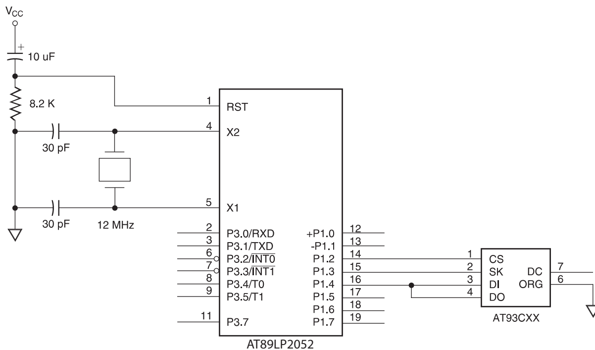
Figure 1-1. 3-Wire Configuration
