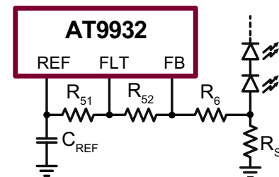
Figure 5. Output Short Circuit Protection
