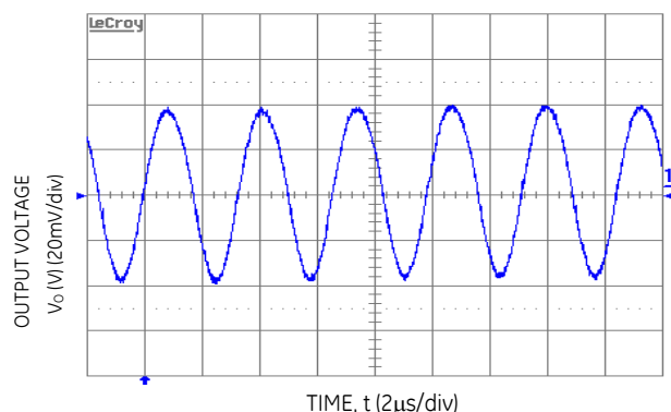
Figure 9. Typical Output Ripple and Noise ( V_{IN} = 12.0Vdc , V_O = 3.3Vdc , I_O = 10A ).
