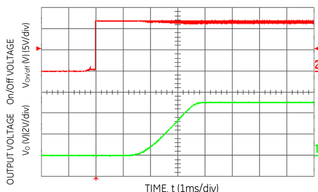
Figure 15. Typical Start-Up Using Remote On/Off with external capacitors ( V_{in} = 12.0\text{ Vdc} , V_o = 5.0\text{ Vdc} , I_o = 10\text{ A} , C_o = 1050\text{ }\mu\text{F} ).
