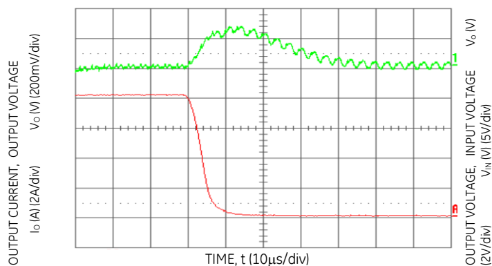
Figure 13. Transient Response to Dynamic Load Change from 100% of 50% full load ( V_o = 3.3\text{Vdc} , C_{ext} = 2 \times 150 \mu\text{F} Polymer Capacitors)
