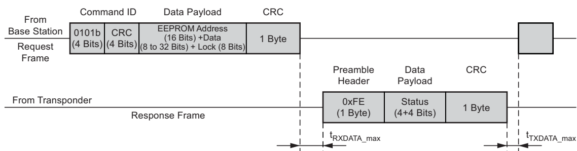
Figure 2-16. The Write User Memory Sequence
