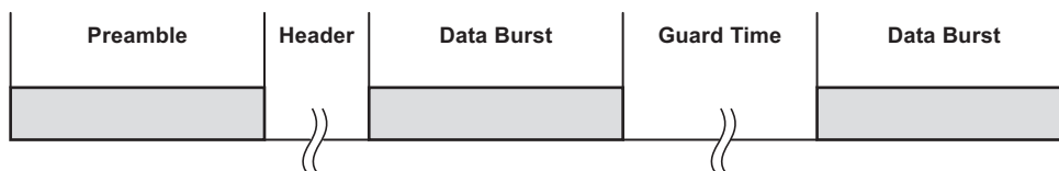
Figure 6-2. Supported Header and Blanking Periods
