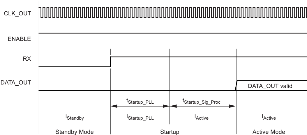
Figure 5-3. Active Mode
