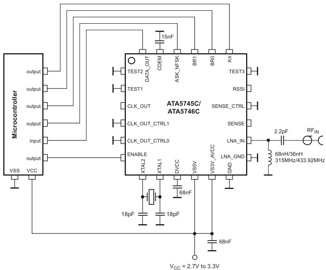
Figure 9-1. 3V Application
