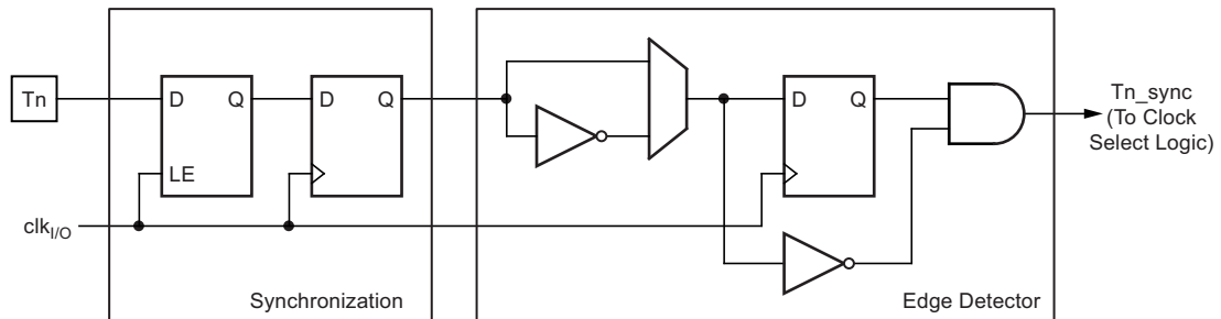
Figure 4-50. T0 Pin Sampling
