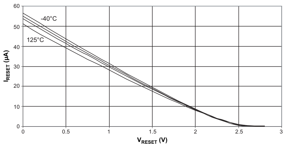
Figure 8-17. Reset Pull-up Resistor Current versus Reset Pin Voltage ( V_{CC} = 2.7V )
