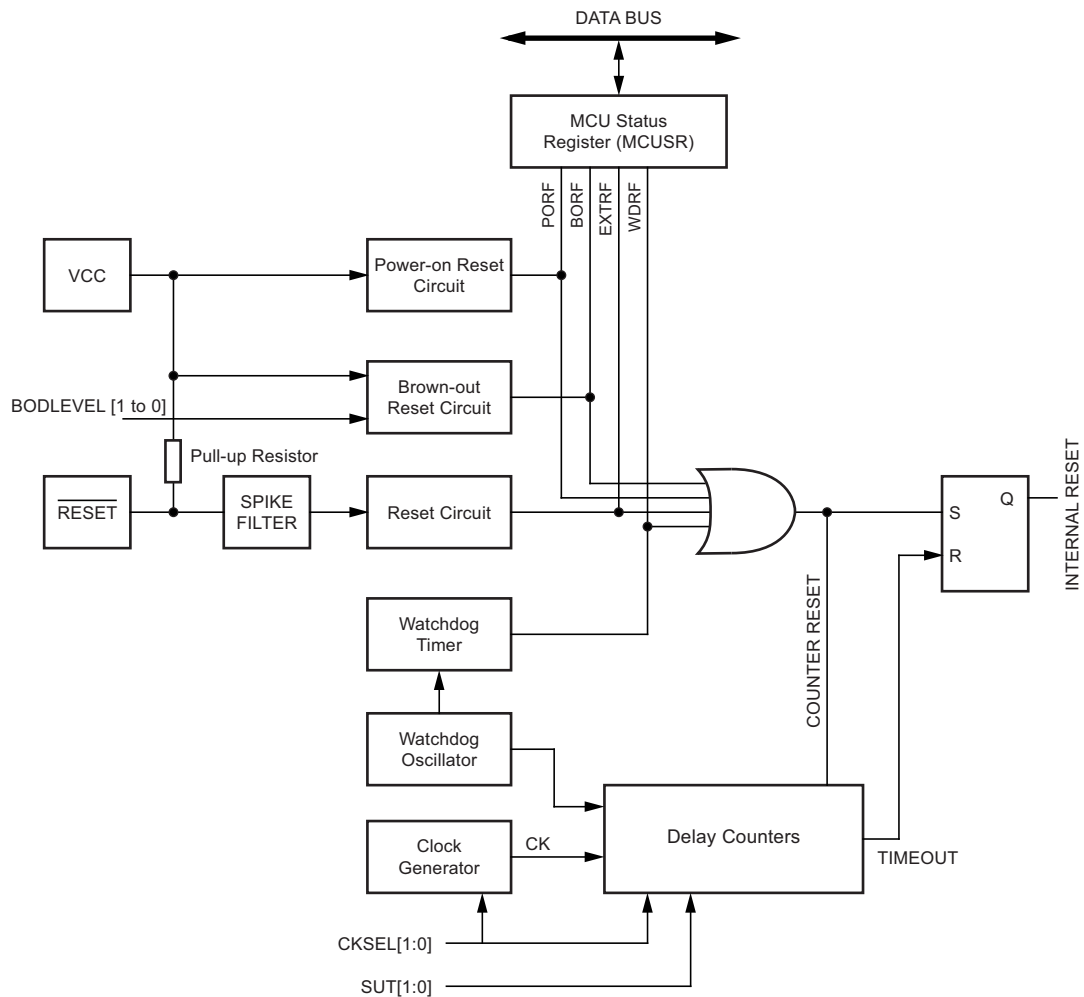
Figure 4-13. Reset Logic
