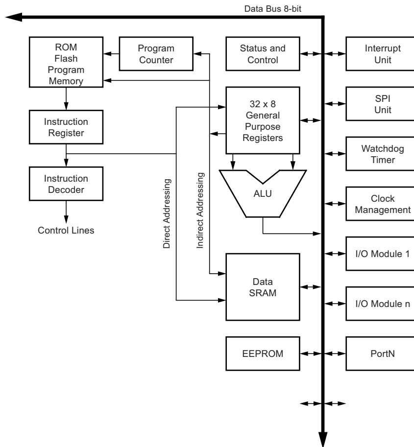
Figure 3-3. Architectural Overview
