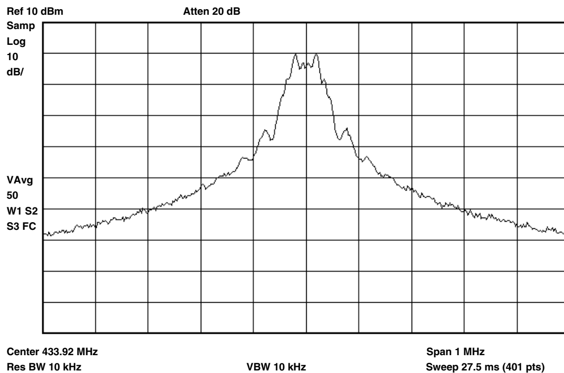
Figure 7-11. FSK-modulated TX Spectrum (433.92 MHz/20 Kbit/s/ \pm 19.41 kHz/Manchester Code)
