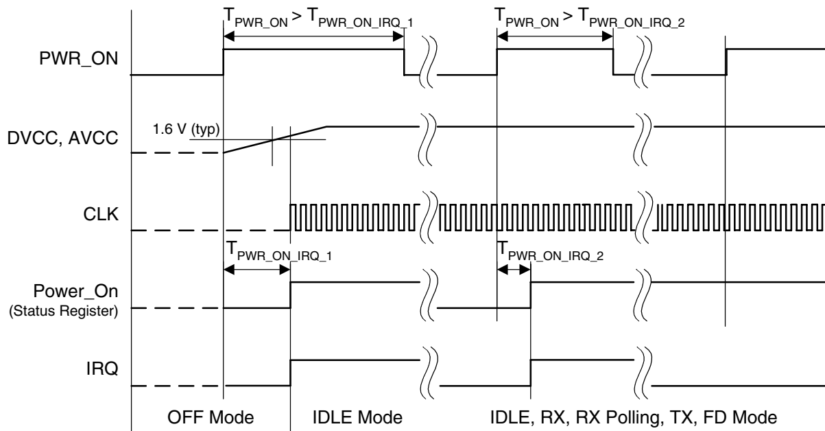
Figure 12-4. Timing Pin \text{PWR\_ON} , Status Bit \text{Power\_On}
