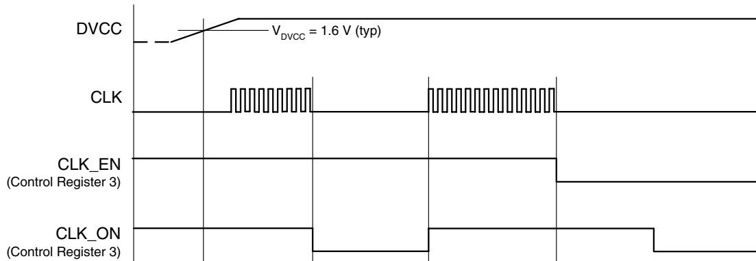
Figure 9-3. Clock Timing
