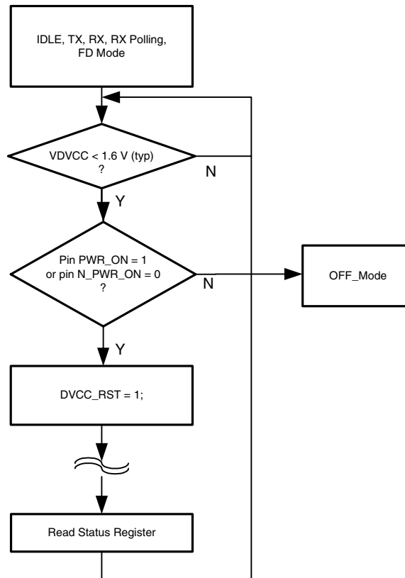
Figure 12-5. Timing Flow Status Bit DVCC_RST
