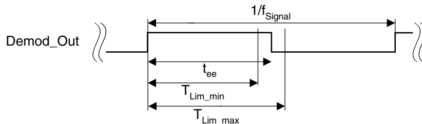
Figure 14-3. Valid Time Window for Bit-check
