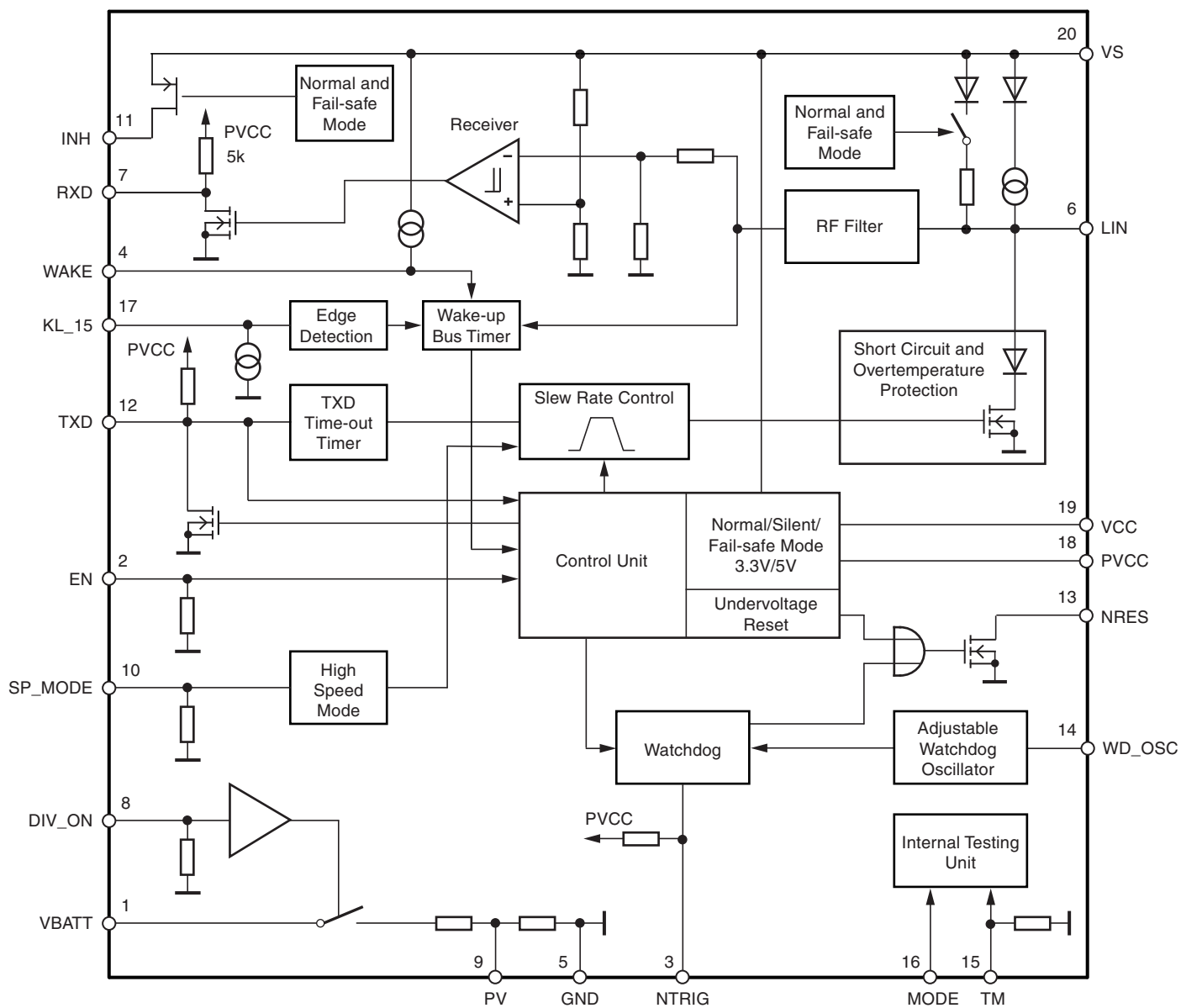
Figure 1-1. Block Diagram
