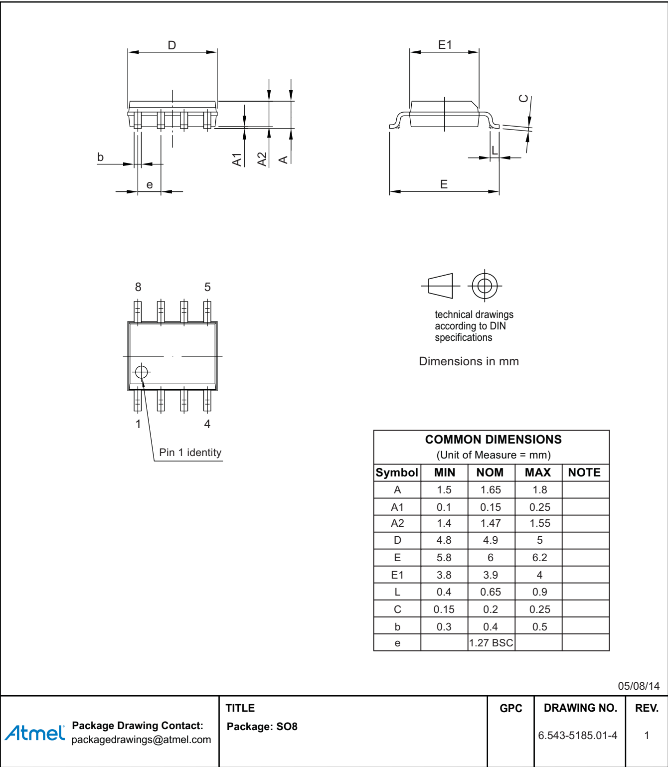
Figure 11-2. SO8
