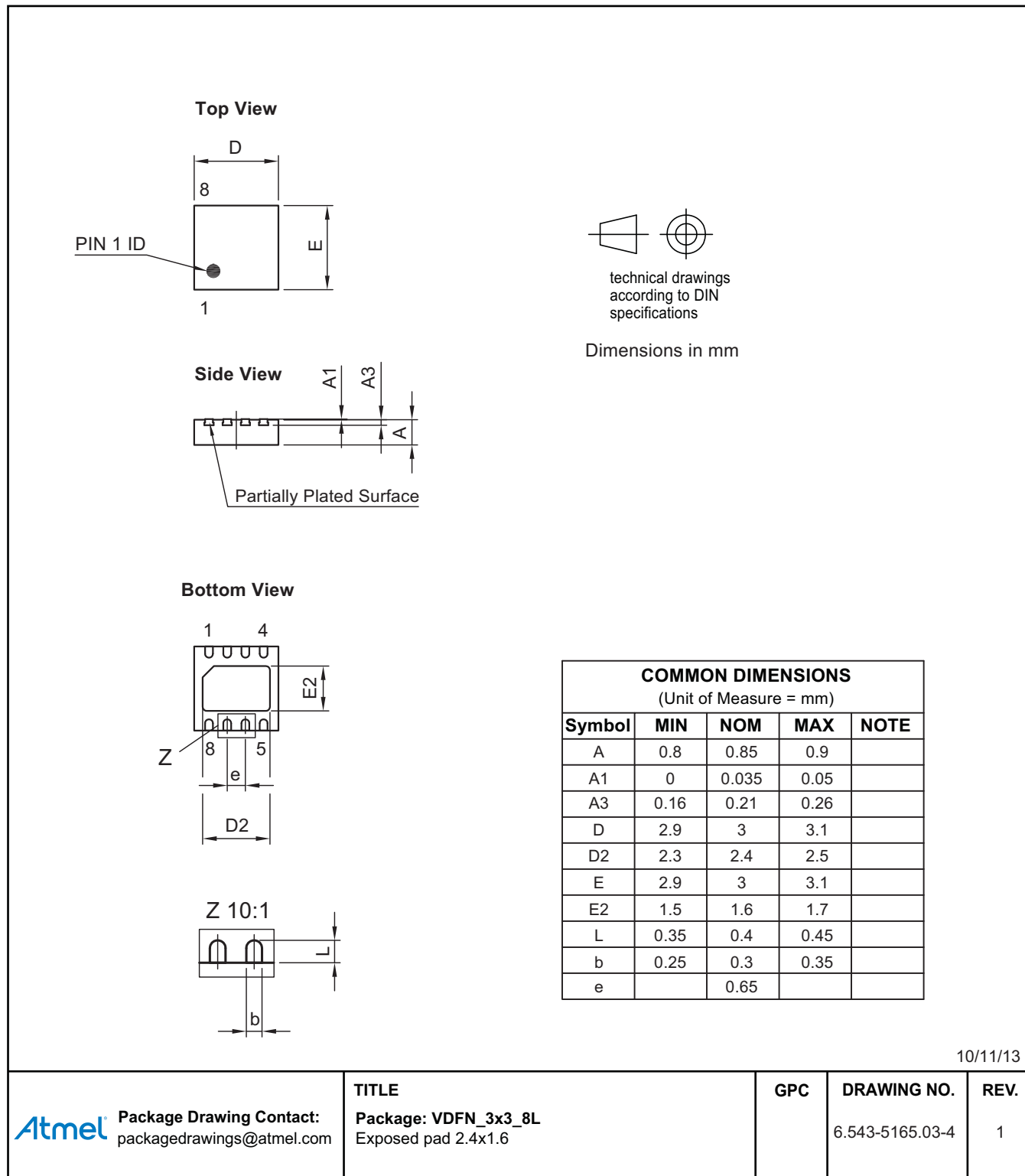
Figure 11-1. DFN8
