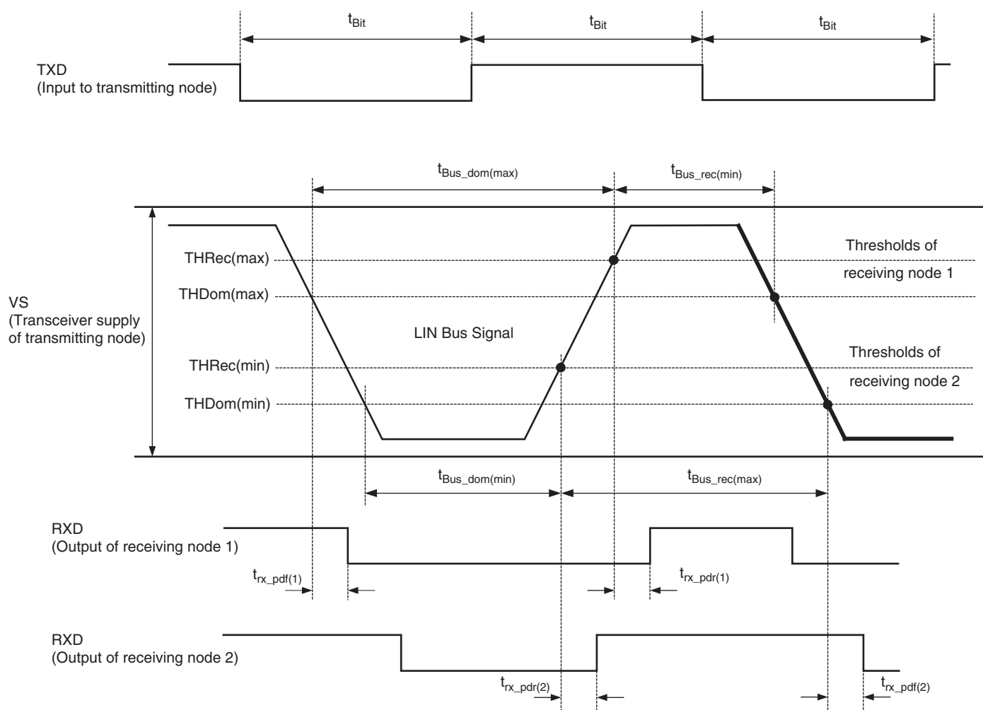
Figure 6-1. Definition of Bus Timing Parameter
