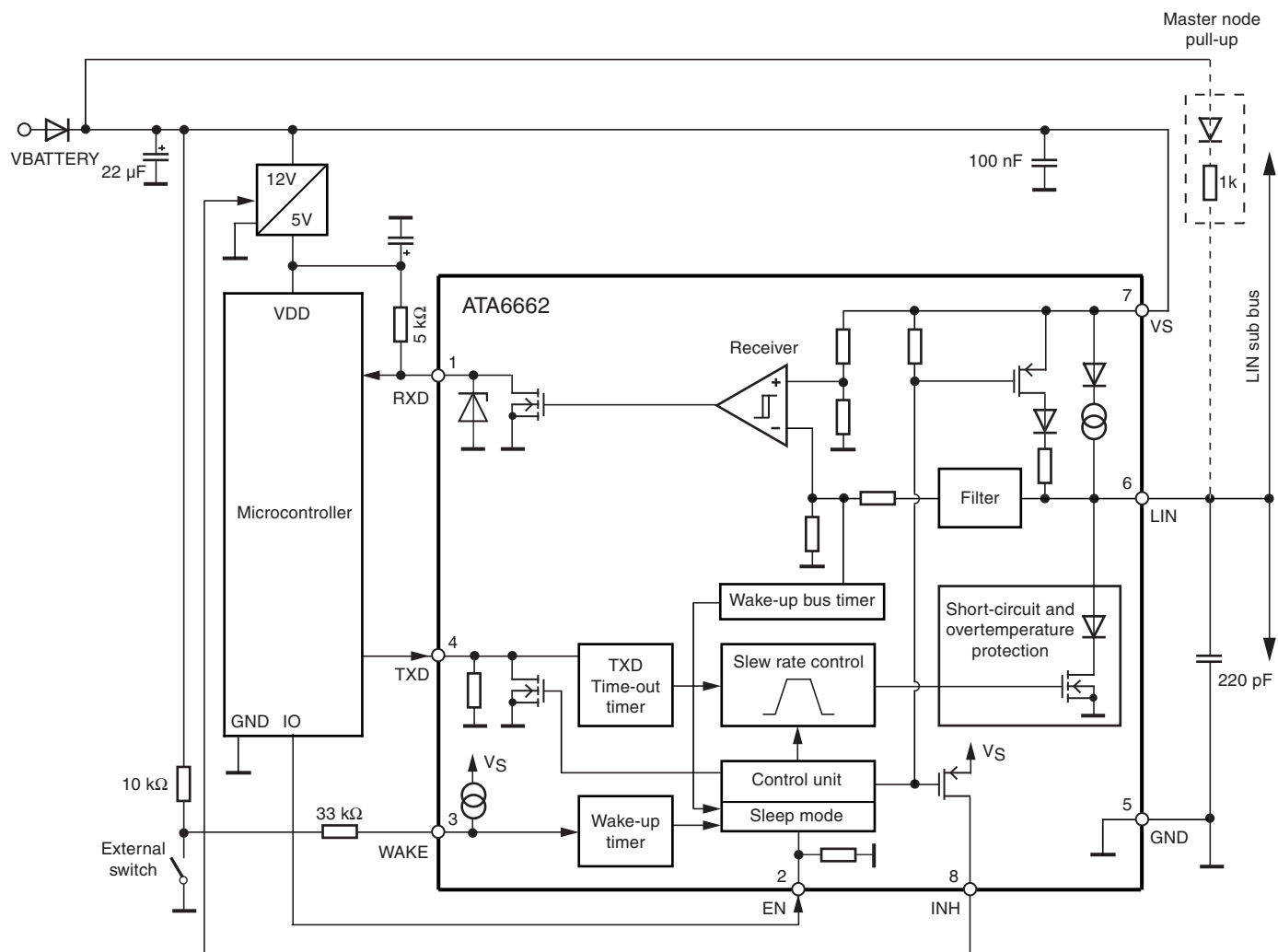
Figure 6-2. Application Circuit
