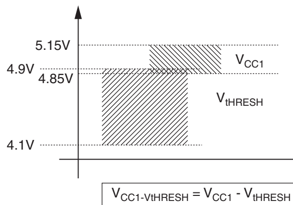
Figure 3-2. Correlation between VCC Output Voltage and Reset Threshold
