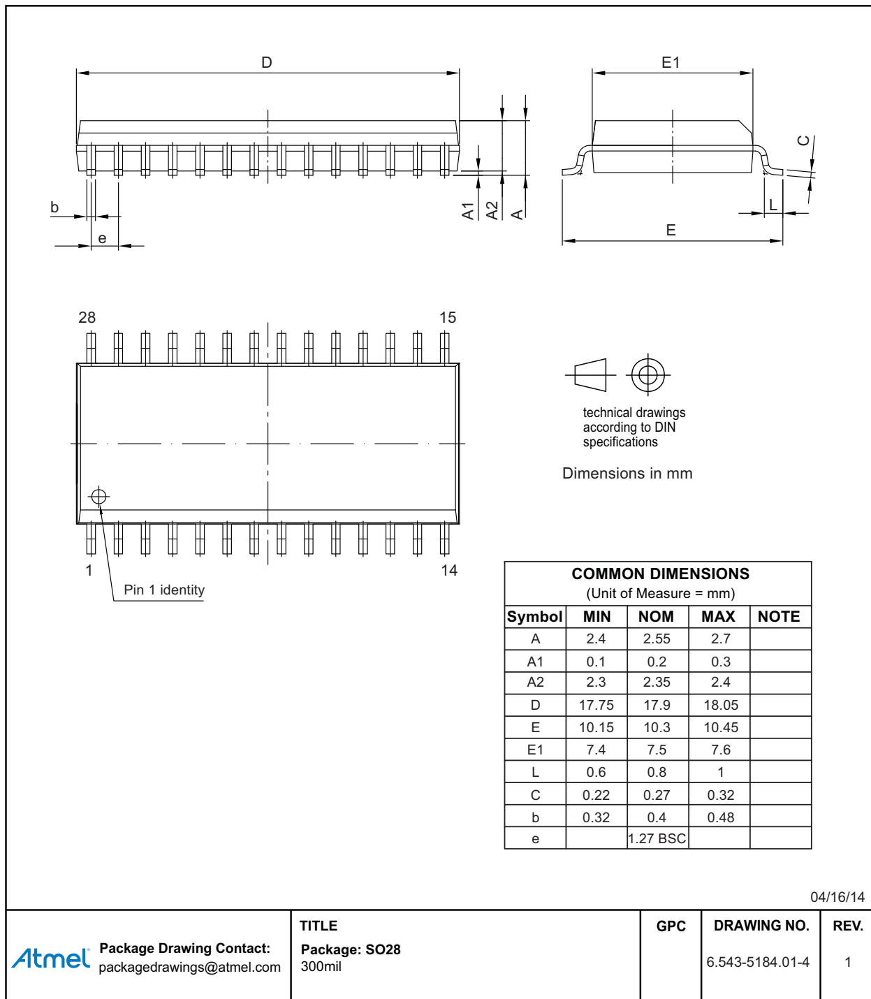
Figure 12-1. SO28
