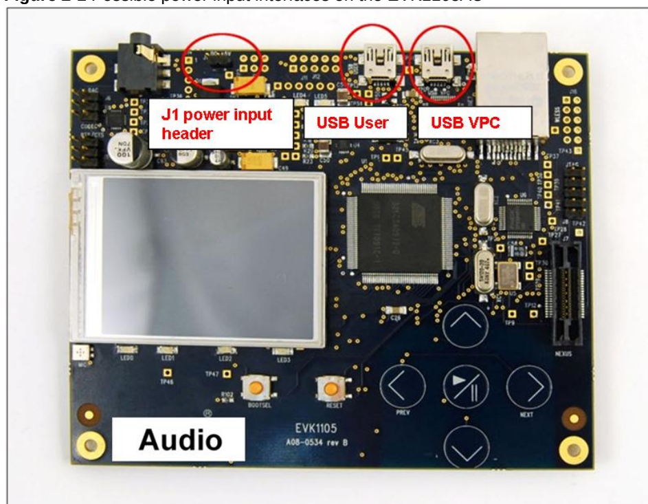
Figure 2-1 Possible power input interfaces on the EVK1105AU
