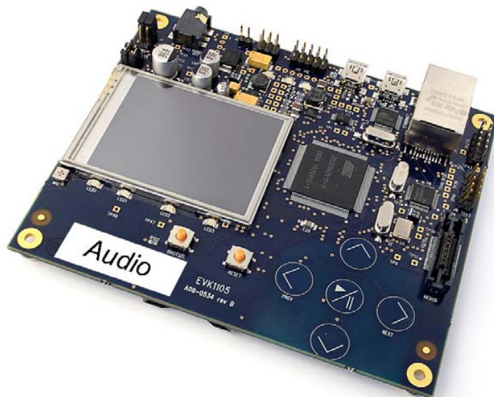
Figure 1-1 EVK1105AU board
