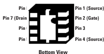
Figure 11. LPCC Package for ATF-521P8.
