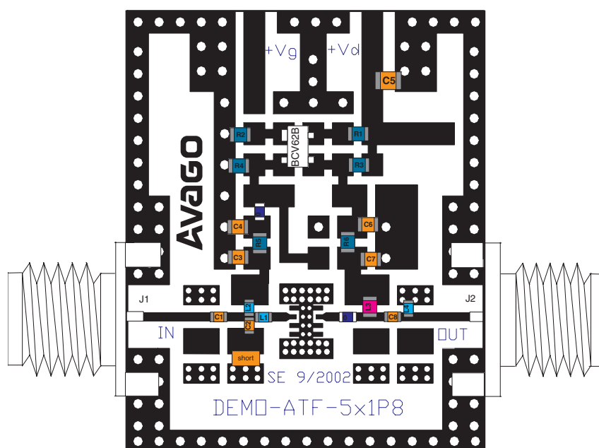
Figure 12. ATF-521P8 demoboard.
