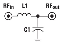
Figure 5. Low Pass Circuit Topology.
