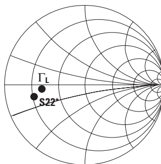
Figure 2. Output Match at 2 GHz.
