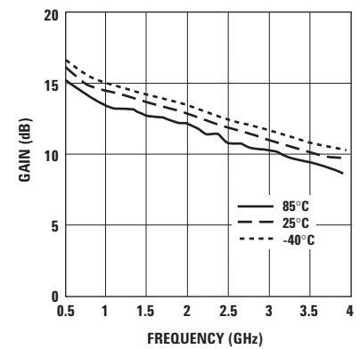
Figure 38. Gain vs. Temp and Freq tuned for optimal P1dB at 4.5V, 200 mA.
