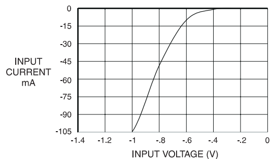
INPUT CLAMP CURRENT vs. INPUT VOLTAGE
