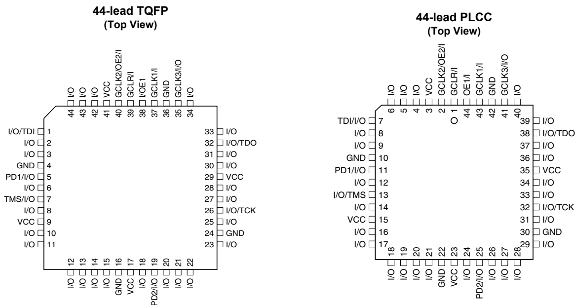
Figure 1-1. Pinouts
