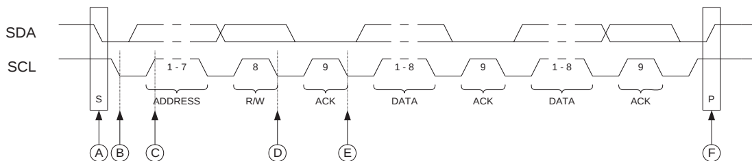
Figure 14-5. Two-wire Mode, Typical Timing Diagram
