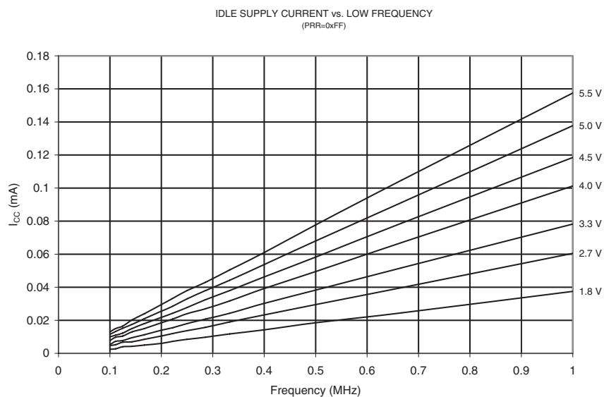
Figure 21-6. Idle Supply Current vs. Low Frequency (0.1 - 1.0 MHz)
