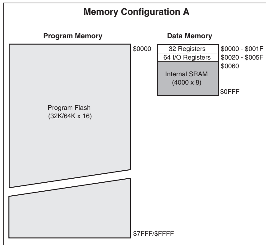
Figure 7. Memory Configurations
