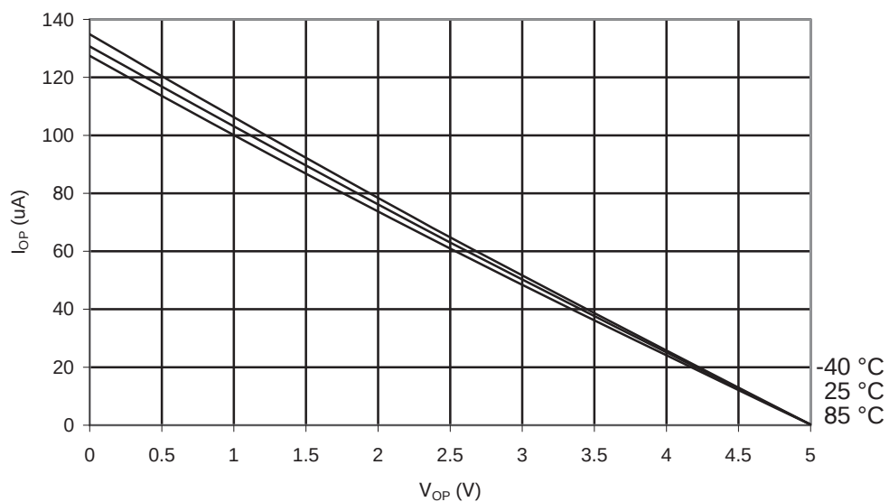
Figure 27-17. ATmega1284P: I/O Pin Pull-up Resistor Current vs. Input Voltage ( V_{CC} = 5V ).
