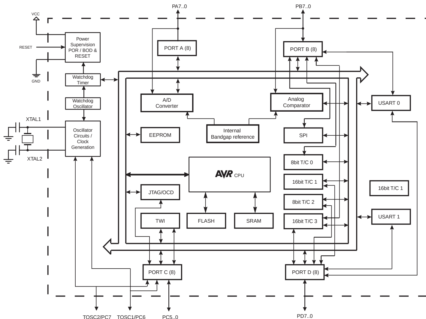
Figure 2-1. Block Diagram
