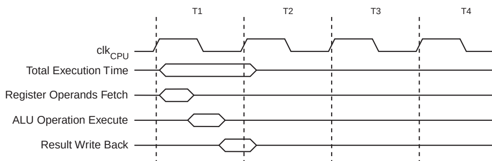
Figure 5-6. Single Cycle ALU Operation
