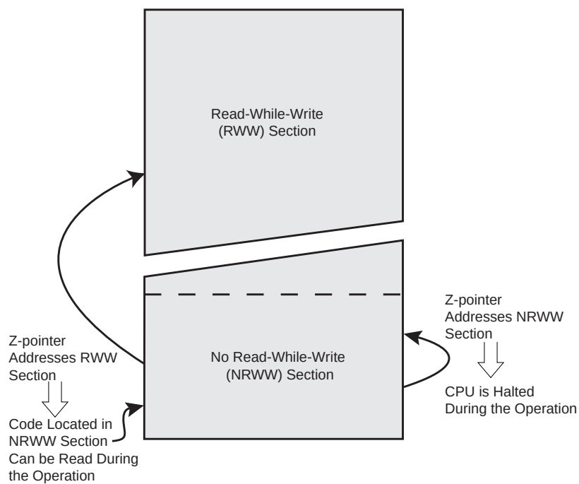
Figure 24-1. Read-While-Write vs. No Read-While-Write
