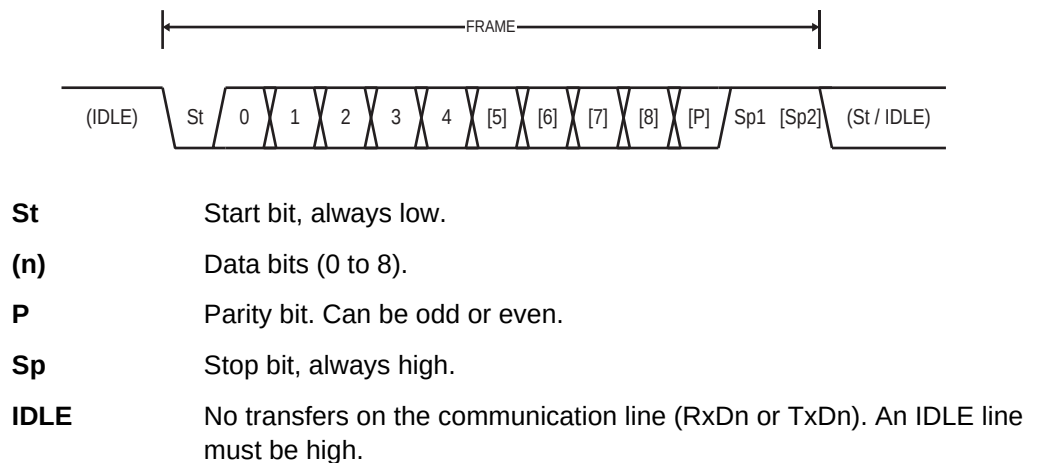
Figure 17-4. Frame Formats
