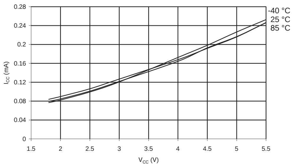
Figure 27-10. ATmega1284P: Idle Supply Current vs. V_{CC} (Internal RC Oscillator, 128 kHz)
