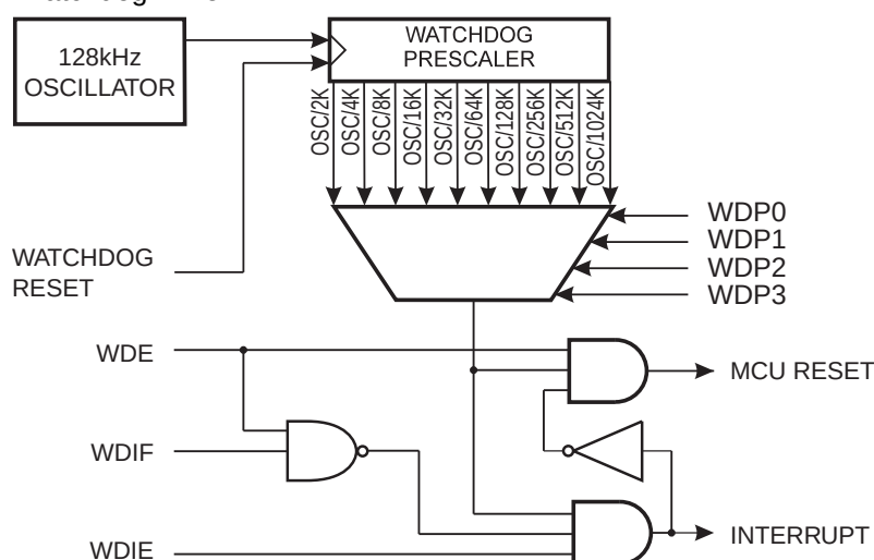
Figure 9-7. Watchdog Timer
