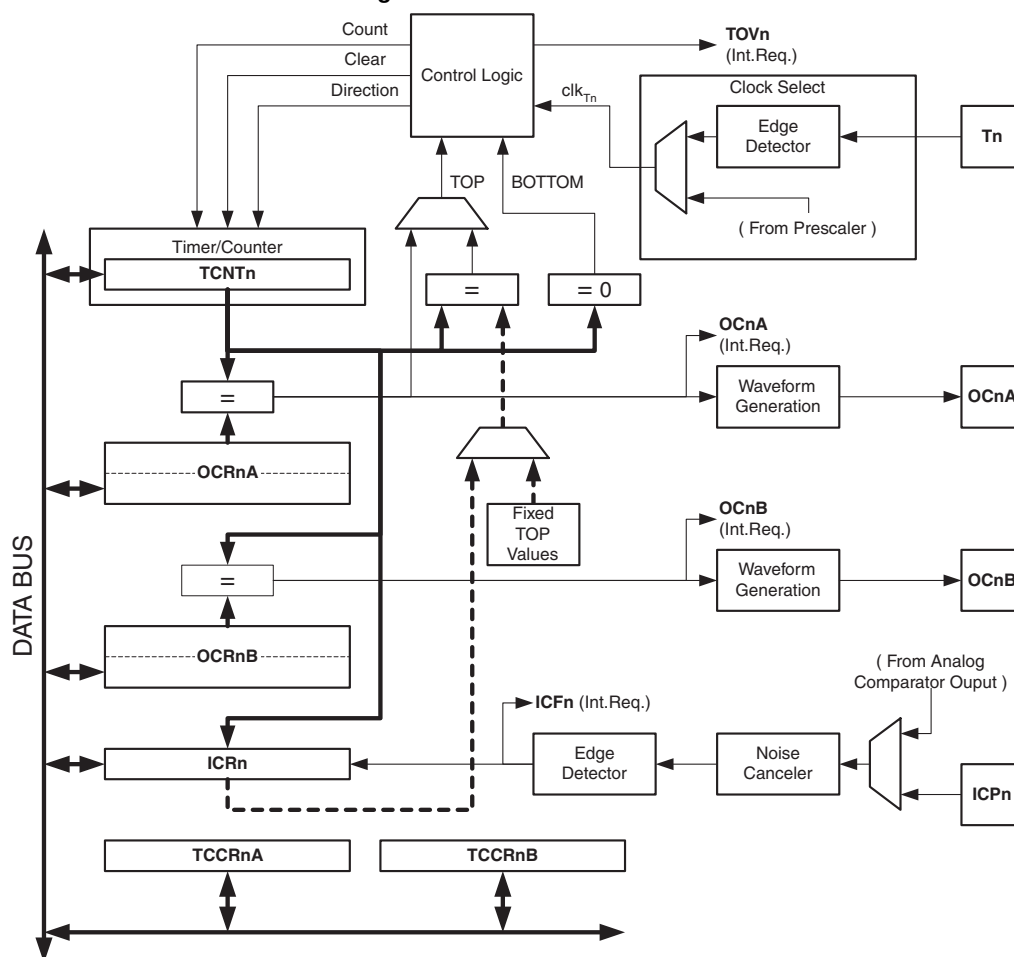
Figure 13-1. 16-bit Timer/Counter Block Diagram (Note:)
