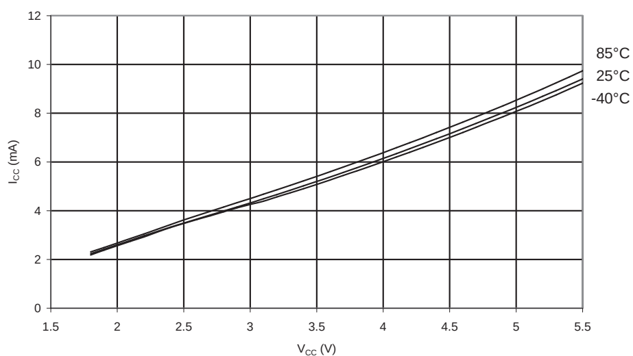
Figure 27-50. Active Supply Current vs. V_{CC} (Internal RC Oscillator, 8 MHz).
