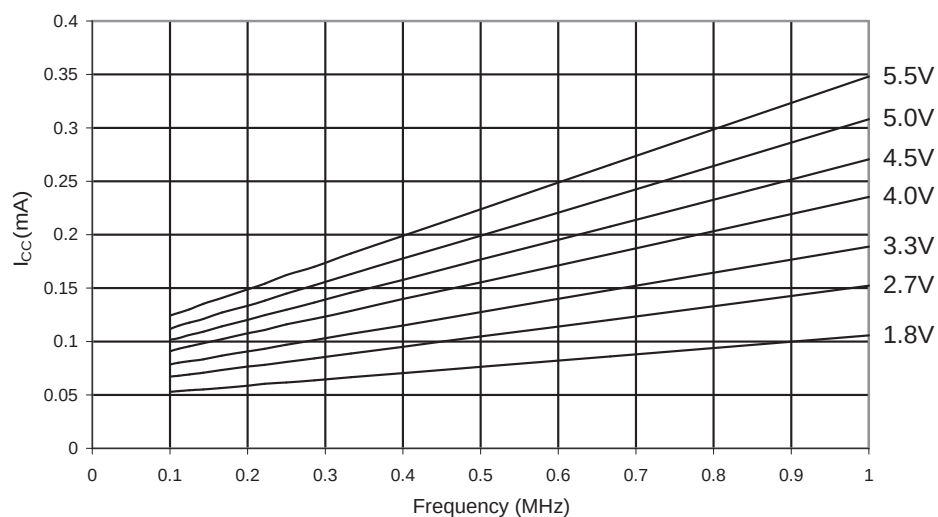
Figure 27-6. Idle Supply Current vs.Low Frequency (0.1 MHz - 1.0 MHz).
