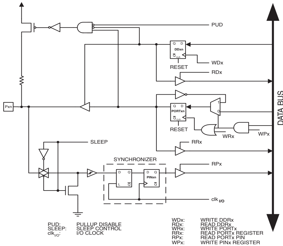
Figure 11-2. General Digital I/O (1)
