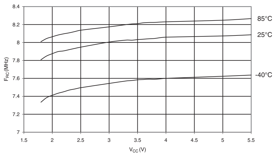
Figure 27-130. Calibrated 8 MHz RC Oscillator vs. V_{CC}
