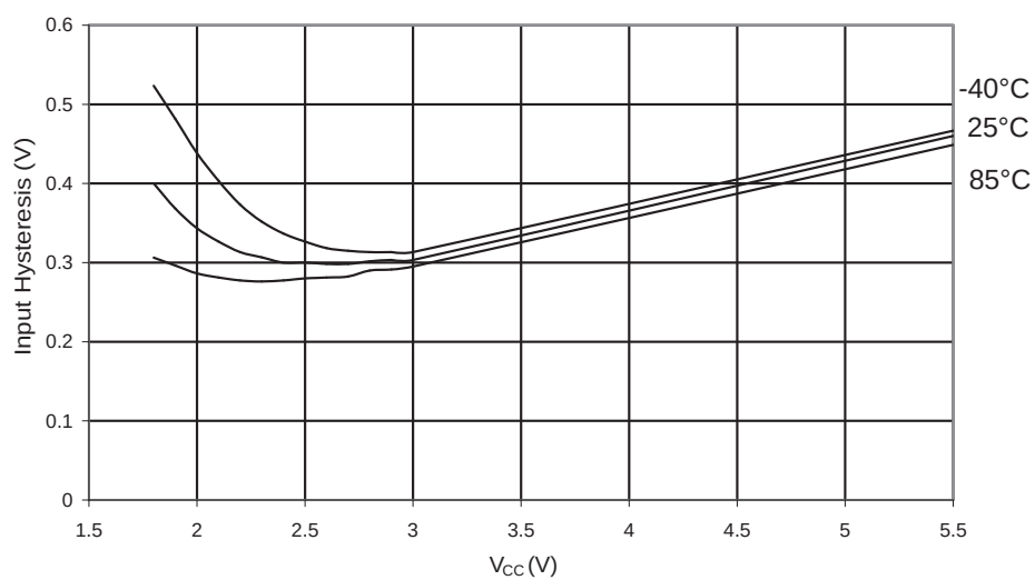
Figure 27-27. I/O Pin Input Hysteresis vs. V_{CC} .
