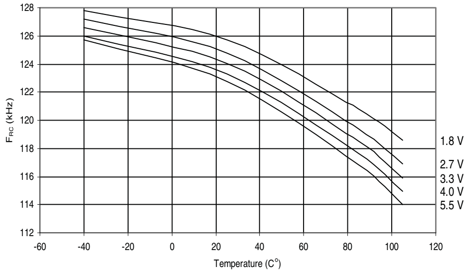
Figure 28-28. ATmega164P: Watchdog Oscillator Frequency vs. Temperature
