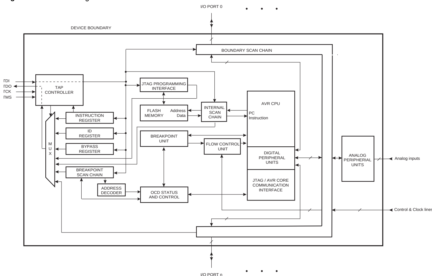
Figure 21-1. Block Diagram
