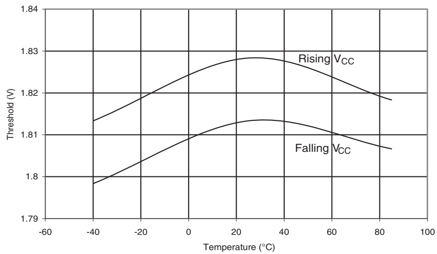
Figure 27-127. BOD Threshold vs. Temperature ( V_{CC} = 1.8V )
