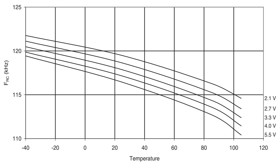
Figure 28-110. ATmega644P: Watchdog Oscillator Frequency vs. Temperature
