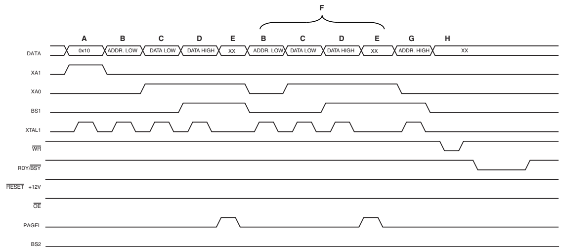
Figure 25-3. Programming the Flash Waveforms (1)
