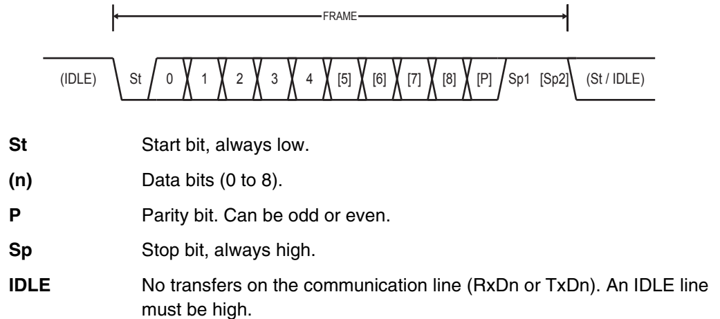
Figure 17-4. Frame Formats
